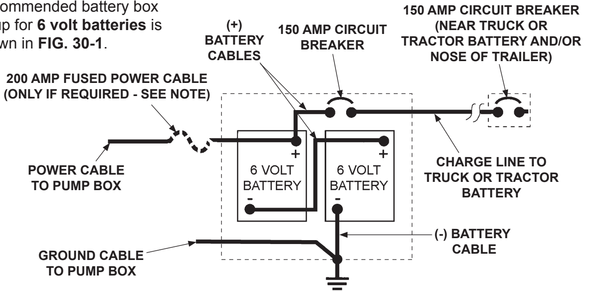
6 VOLT BATTERY CONNECTIONS FIG. 30-1
