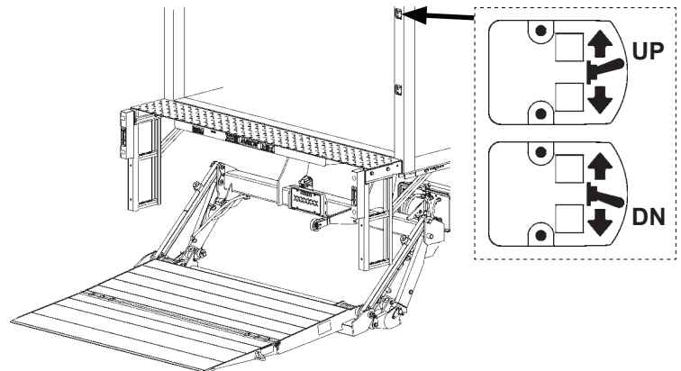
VERIFYING DUAL CONTROL SWITCH FIG. 8-2
