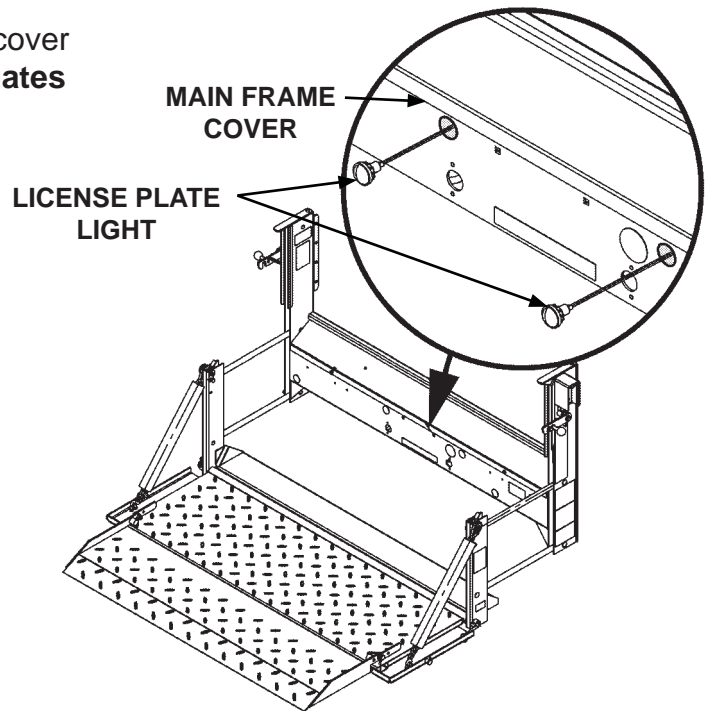
INSTALLING LICENSE PLATE LIGHTS ON C1 LIFTGATE
