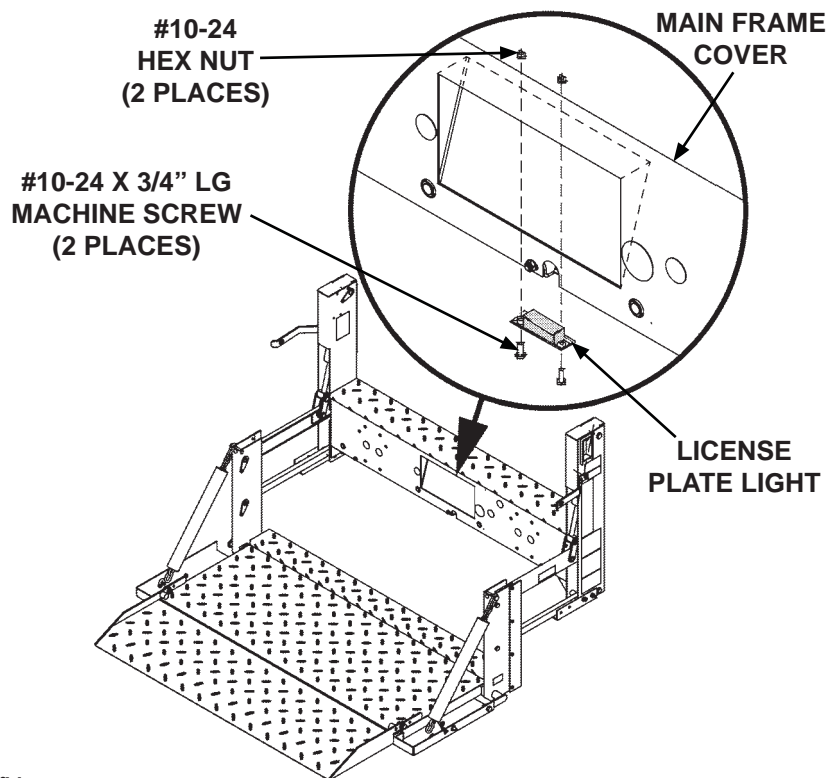
INSTALLING LICENSE PLATE LIGHTS ON C2 LIFTGATE
