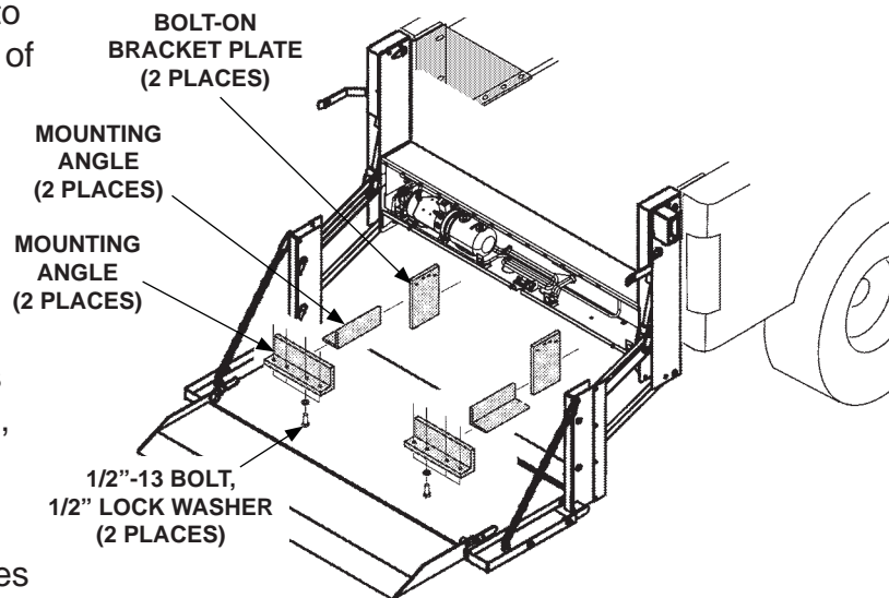
FABRICATING LOWER BRACKETS TO SUPPORT LIFTGATE (C2 SHOWN) FIG. 15-2
