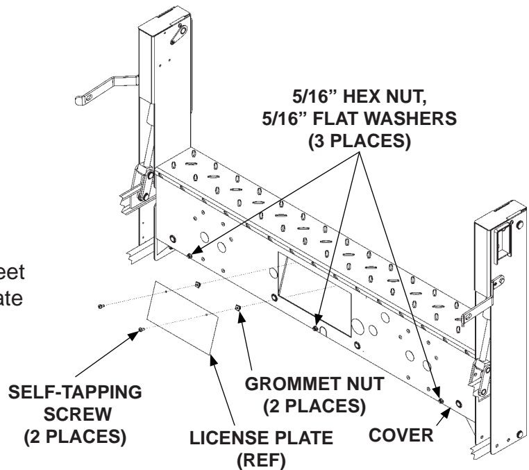
INSTALLING COVER & LICENSE PLATE (C2 LIFTGATE SHOWN) FIG. 19-2
