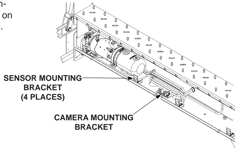
CAMERA AND SENSOR BRACKET LOCATION FIG. 16-1
