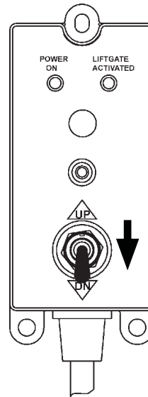
USING CONTROL SWITCH TO LOWER LIFTGATE FIG. 11-1
