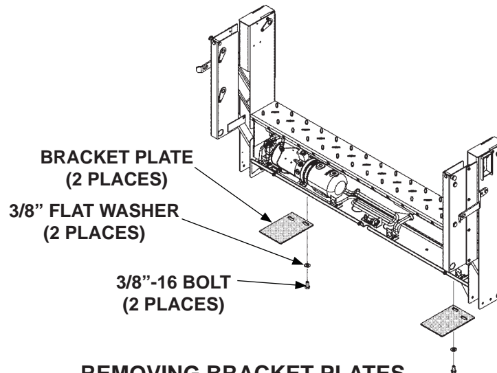
REMOVING BRACKET PLATES (PLATFORM NOT SHOWN) FIG. 5-2
