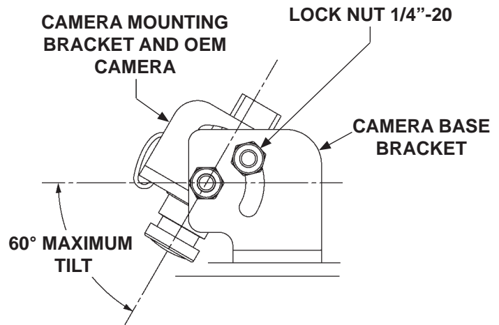
ADJUSTING CAMERA ANGLE FIG. 17-1
