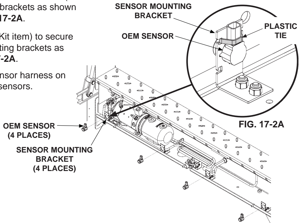
INSTALLING SENSORS (IF EQUIPPED) FIG. 17-2
