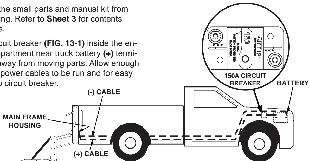
RUNNING POWER CABLES FROM LIFTGATE TO BATTERY FIG. 13-1
