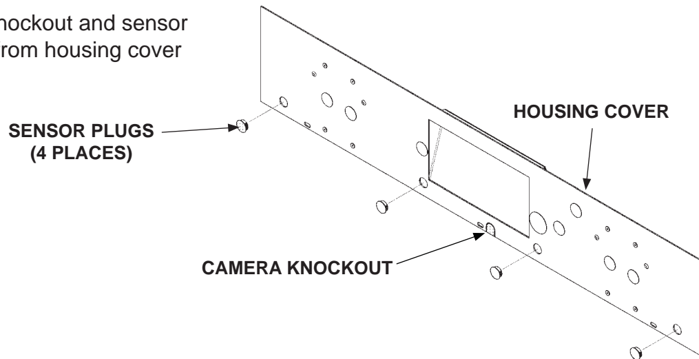
REMOVING HOUSING COVER SENSOR PLUGS AND CAMERA KNOCKOUT FIG. 18-1
