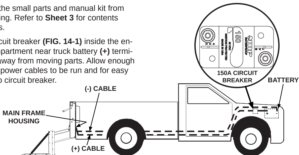
RUNNING POWER CABLES FROM LIFTGATE TO BATTERY
