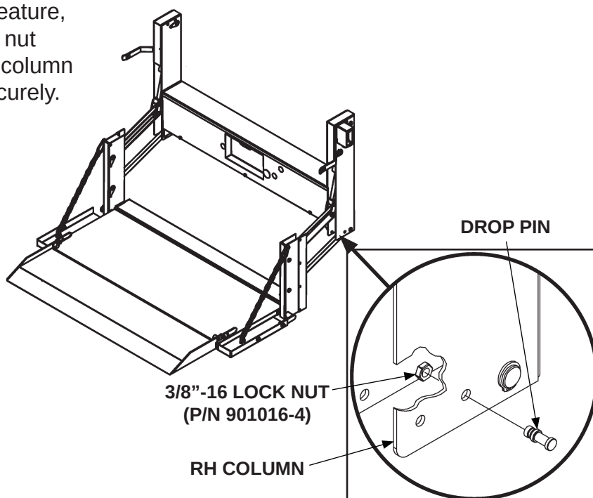
INSTALLING DROP PIN ON RH COLUMN (C2 LIFTGATE SHOWN) FIG. 18-1
