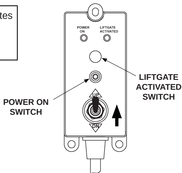
CHECKING OPERATION OF CONTROL SWITCH AND RAISING PLATFORM FIG. 19-1
