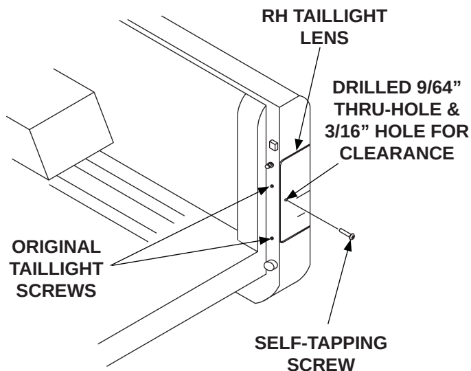
MODIFYING TAILLIGHT MOUNTING FIG. 8-1
