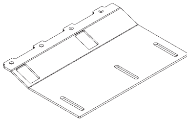
LH MAIN FRAME MOUNTING BRACKET, GALVANIZED P/N 299929-01G QTY. 1
