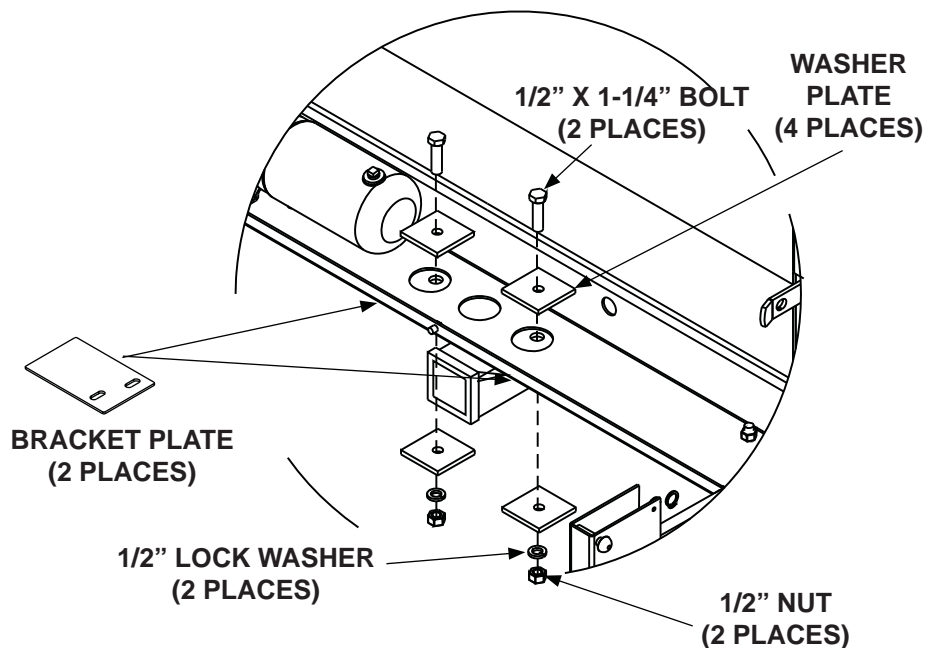
INSTALLING WASHER PLATE ON CLASS 5 HITCH FIG. 24-2
