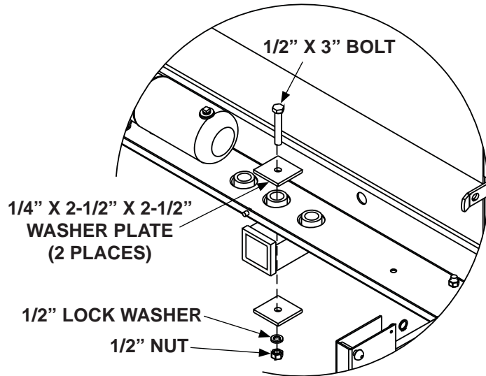
INSTALLING WASHER PLATE ON CLASS 4 HITCH FIG. 24-1
