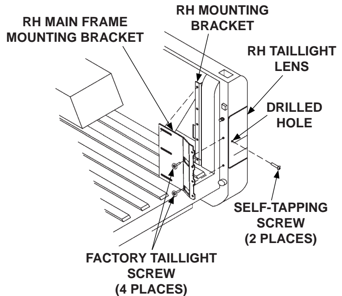
MODIFYING TAILLIGHT MOUNTING FIG. 11-1
