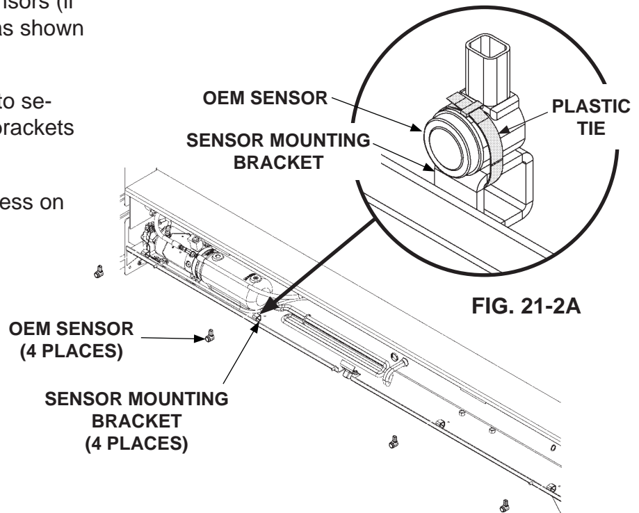
INSTALLING SENSORS (IF EQUIPPED) FIG. 21-2
