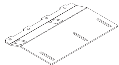
RH MAIN FRAME MOUNTING BRACKET, GALVANIZED P/N 299929-02G QTY. 1
