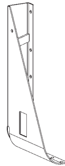
RH MOUNTING BRACKET, GALVANIZED P/N 299943-02G QTY. 1
