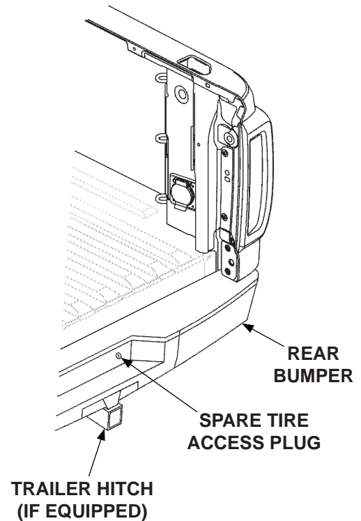
REMOVING TAILGATE AND REAR BUMPER FIG. 14-1
