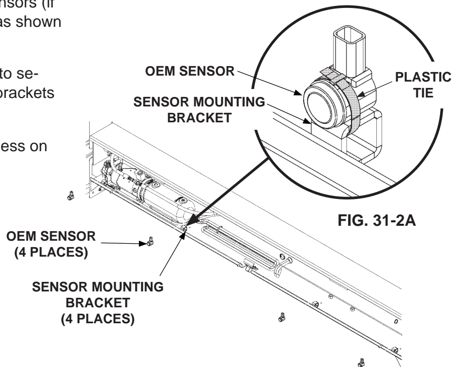
INSTALLING SENSORS (IF EQUIPPED) FIG. 31-2
