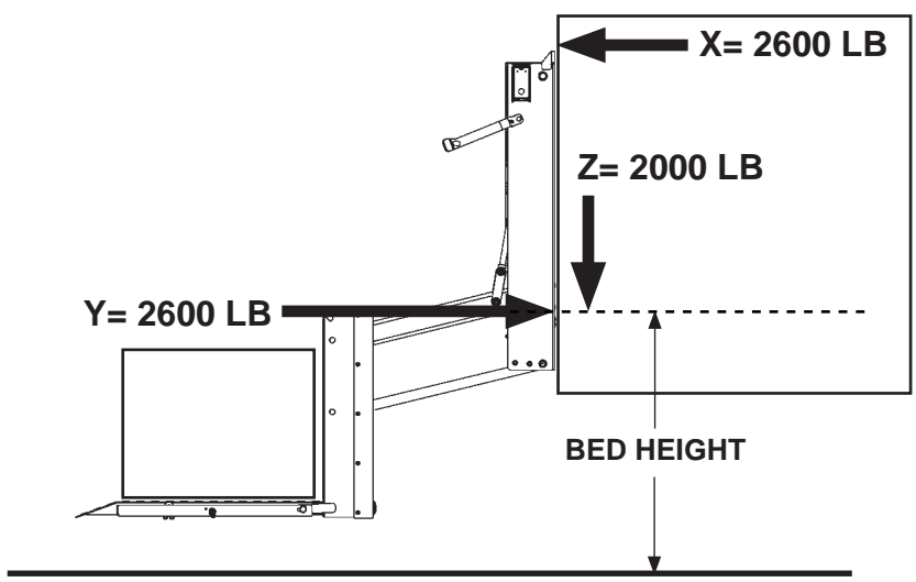
C2 LIFTGATE SHOWN ON TRUCK BODY FIG. 9-1
