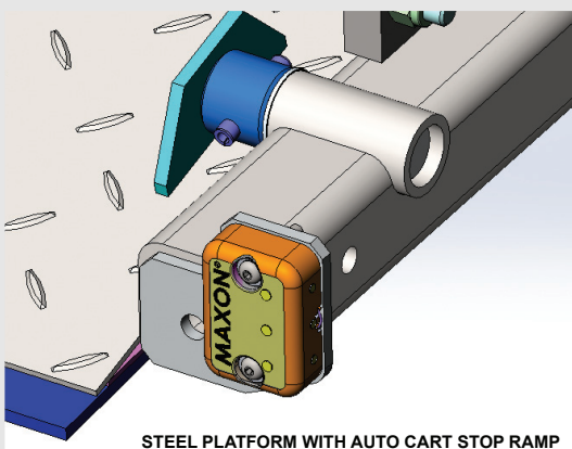
STEEL PLATFORM WITH AUTO CART STOP RAMP
