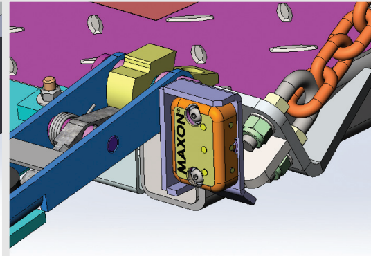
STEEL PLATFORM WITH ALUMINUM RETENTION RAMP
