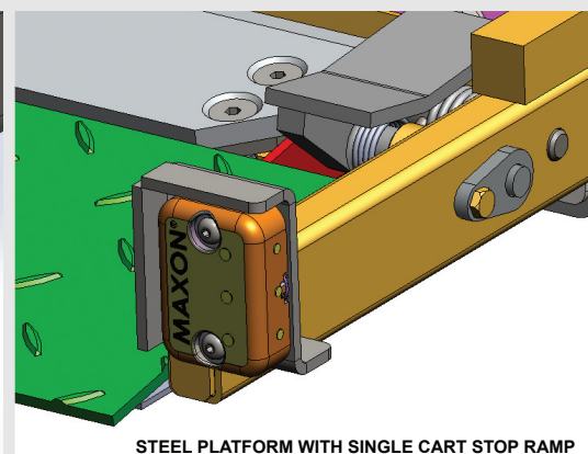
STEEL PLATFORM WITH SINGLE CART STOP RAMP
