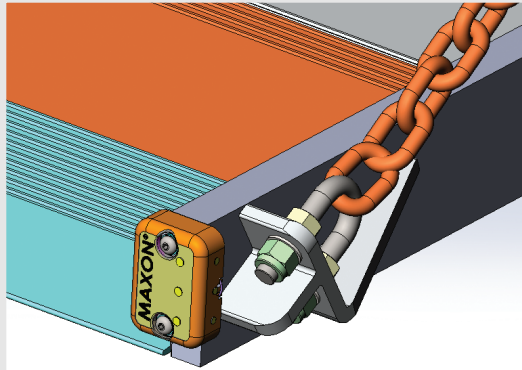
ALUMINUM PLATFORM WITH FIXED RAMP
