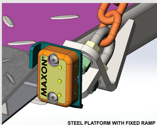
STEEL PLATFORM WITH FIXED RAMP
