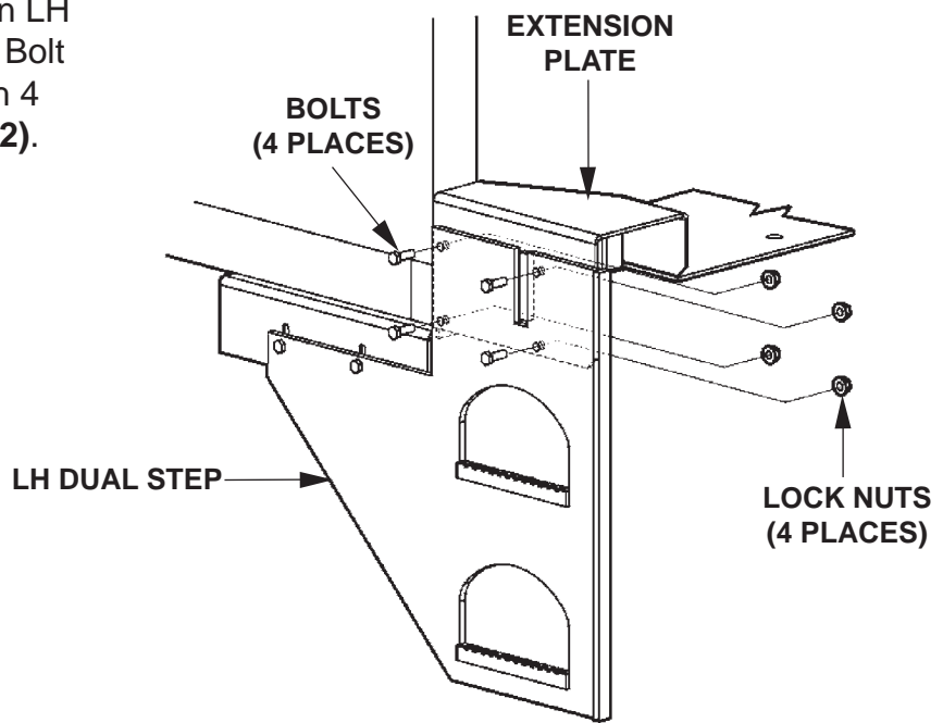
BOLTING ON THE LH DUAL STEP FIG. 9-2
