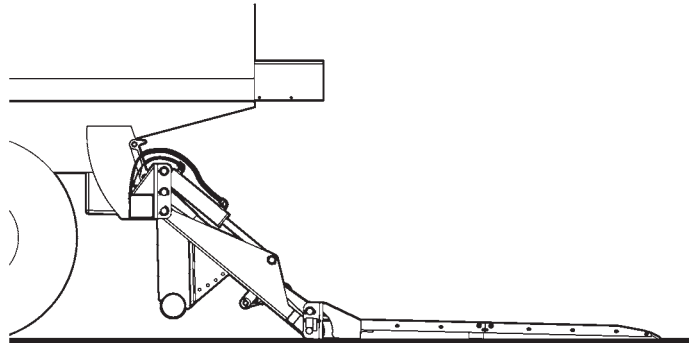
PLATFORM AT GROUND LEVEL (LH SIDE SHOWN) FIG. 9-1
