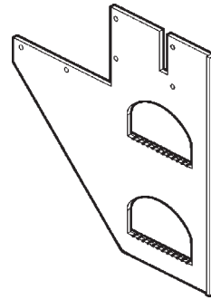
DUAL STEP, RH P/N 281313-02G QTY. 1
