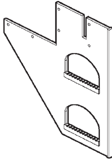
DUAL STEP, LH P/N 281299-01 QTY. 1
