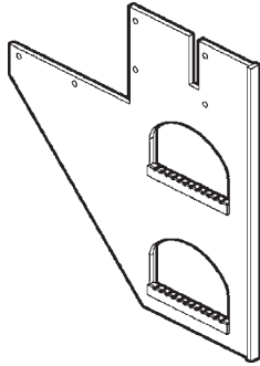
DUAL STEP, LH P/N 281299-01G QTY. 1
