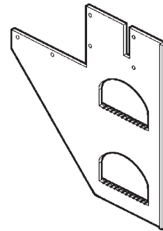
DUAL STEP, RH P/N 281299-02 QTY. 1
