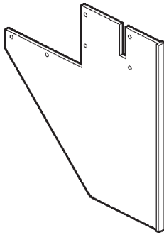
SIDE PLATE, LH (NO STEPS) P/N 281313-03 QTY. 1
