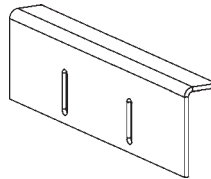
STEP HOLDER ANGLE P/N 281099-01G QTY. 2
