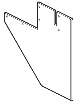
SIDE PLATE, RH (NO STEPS) P/N 281313-04 QTY. 1
