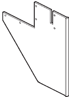
SIDE PLATE, LH (NO STEPS) P/N 281313-03G QTY. 1
