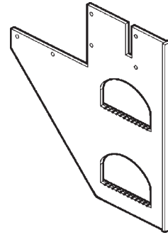
DUAL STEP, RH P/N 281299-02G QTY. 1
