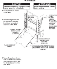
STEP 16 - FINISH WELDING LIFTGATE TO VEHICLE - Continued
