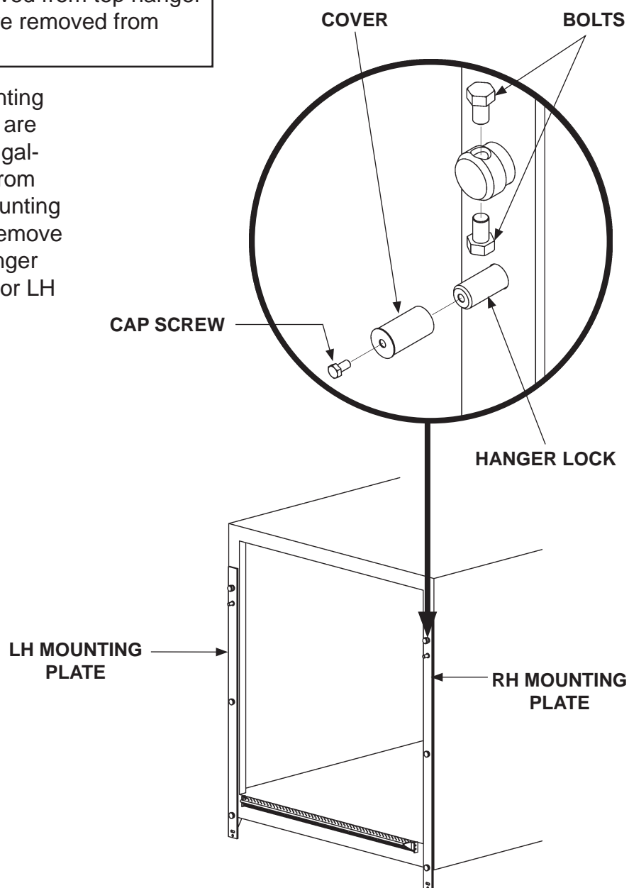
LIFTGATE MOUNTING PLATES FIG. 33-1
