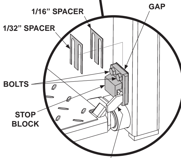
MOUNTING BRACKET
