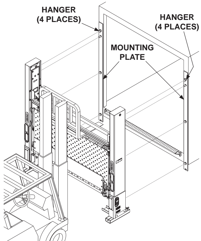
HANGING LIFTGATE FIG. 34-1
