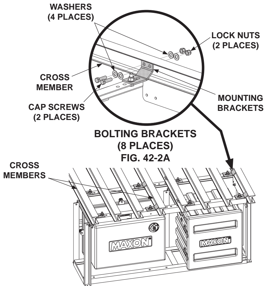
BOLTING PUMP & BATTERY BOX FRAME FIG. 42-2
