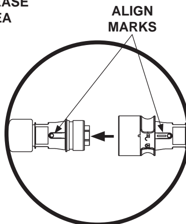
ALIGN & CONNECT FIG. 52-5
