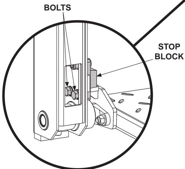
FRONT VIEW OF LH RUNNER FIG. 68-1B
