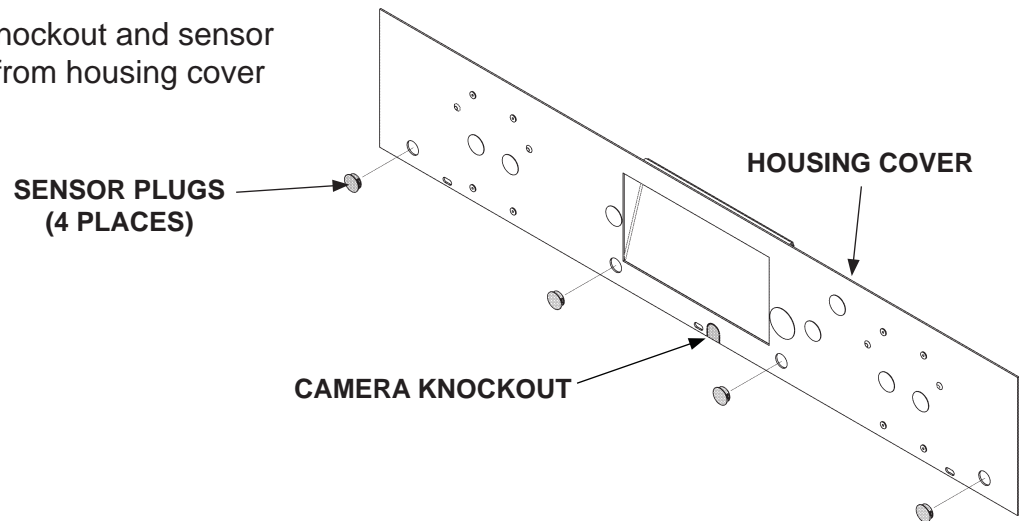
REMOVING HOUSING COVER SENSOR PLUGS AND CAMERA KNOCKOUT FIG. 23-1
