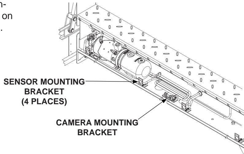
CAMERA AND SENSOR BRACKET LOCATION FIG. 21-1
