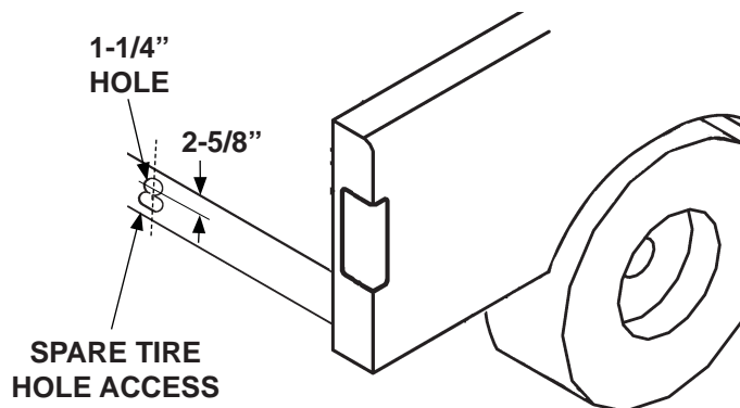
DRILLING HOLE FOR SPARE TIRE CRANK MECHANISM FIG. 11-2
