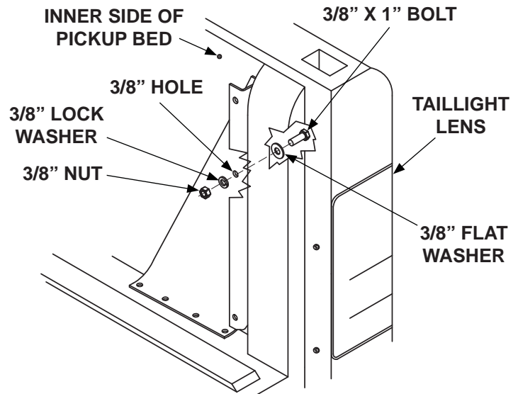
FASTENING BRACKET TO PICKUP BED (RIGHT SIDE SHOWN)
