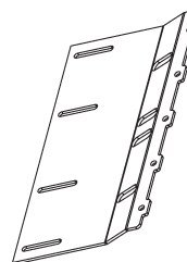
MAIN FRAME MOUNTING BRACKET (GALVANIZED) P/N 289457-01G QTY. 2
