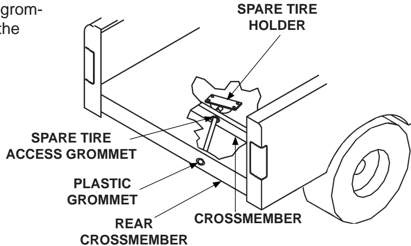
REMOVING GROMMETS FROM FRAME CROSSMEMBERS FIG. 11-1
