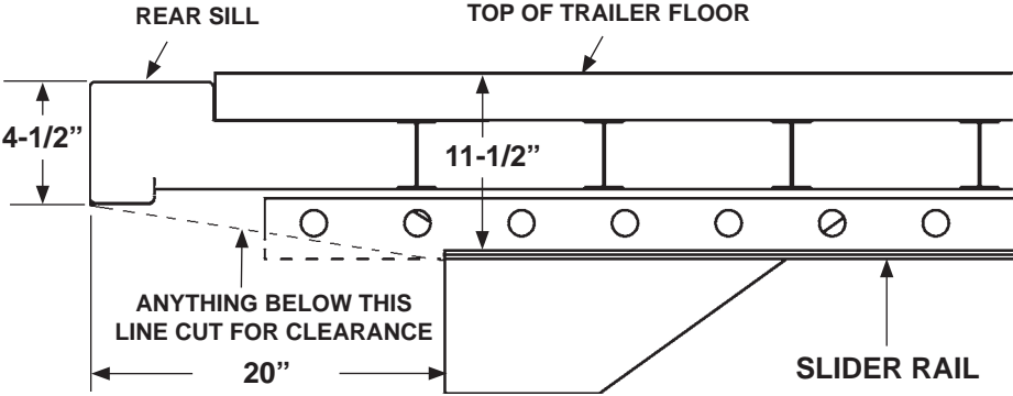
MINIMUM CHASSIS CUT FOR STANDARD TRAILER FIG. 2-1
