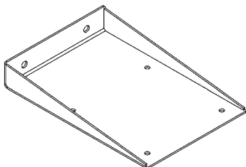
PLACA ANGULAR P/N 263264-01 CANT. 1
