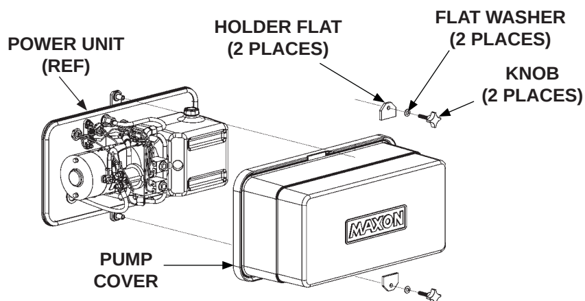
UNBOLTING AND REMOVING PUMP COVER FIG. 7-1
