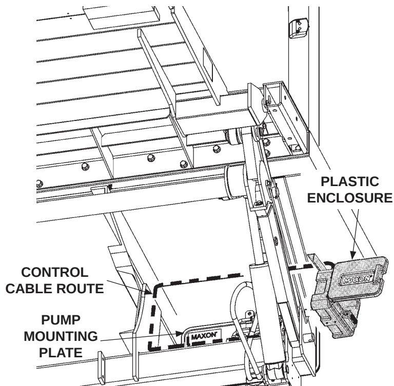
ROUTING ELECTRICAL CABLE UNDER VEHICLE BODY FIG. 7-2
