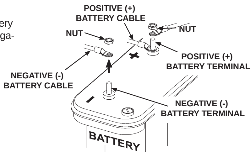
DISCONNECTING (-) BATTERY CABLE FIG. 4-1
