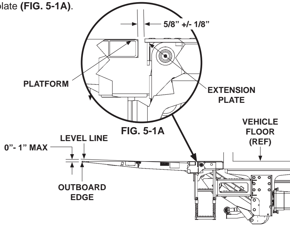
CHECKING PLATFORM FIG. 5-1
