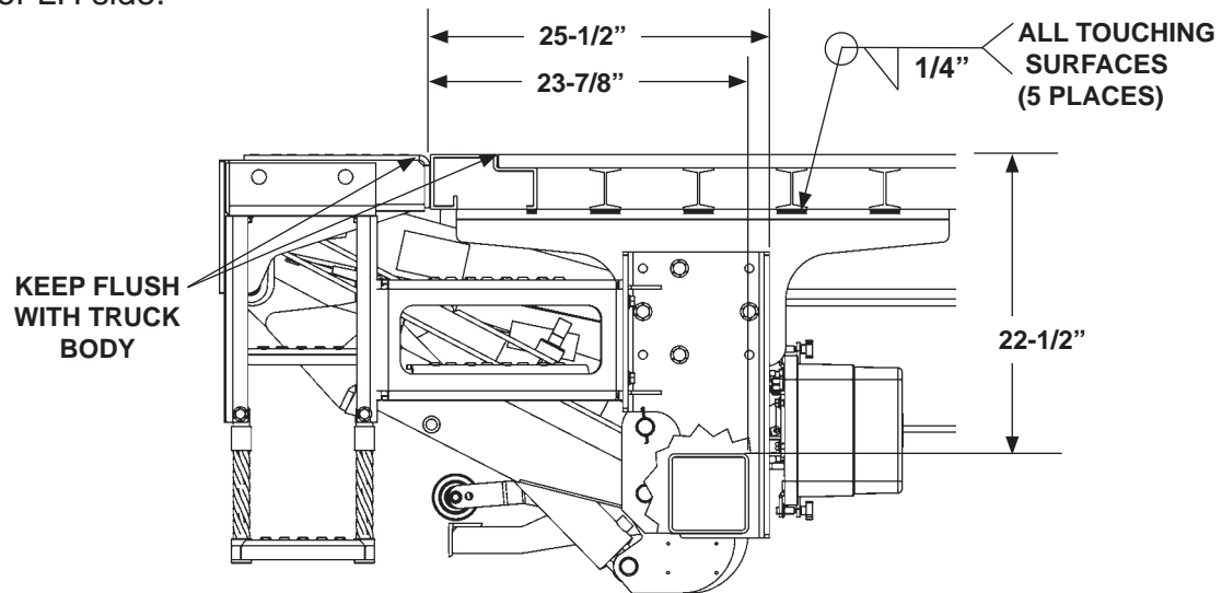
WELDING LIFTGATE TO VEHICLE CHASSIS (RH SIDE SHOWN) FIG. 2-1
