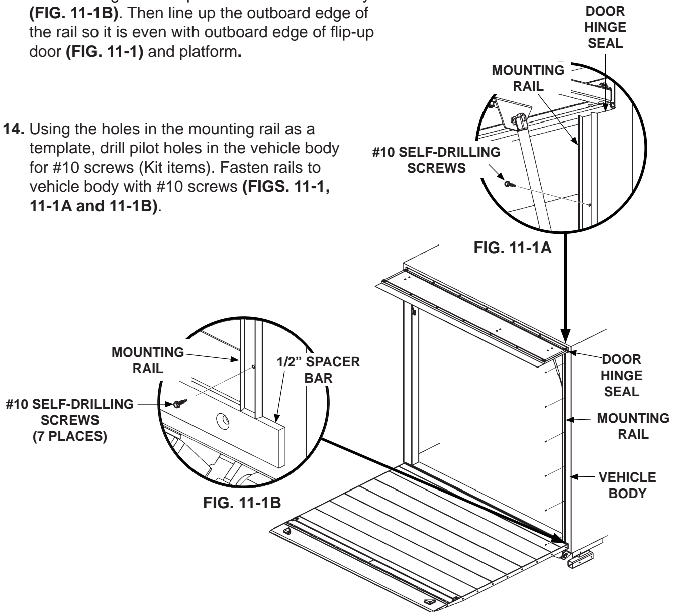
INSTALLING MOUNTING RAILS FIG. 11-1
