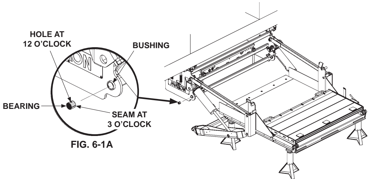
INSTALLING NEW BEARING (LH SIDE SHOWN) FIG. 6-1
