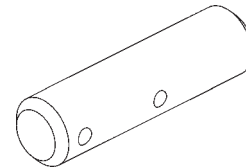
GREASED PIN, 1" X 3-3/4" LG. P/N 283730-02 QTY. 4
