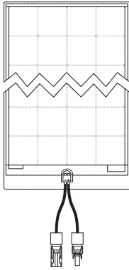
4 X 12 SOLAR PANEL WITH JBOX CABLES, 240W P/N 211628-01 QTY. 1
