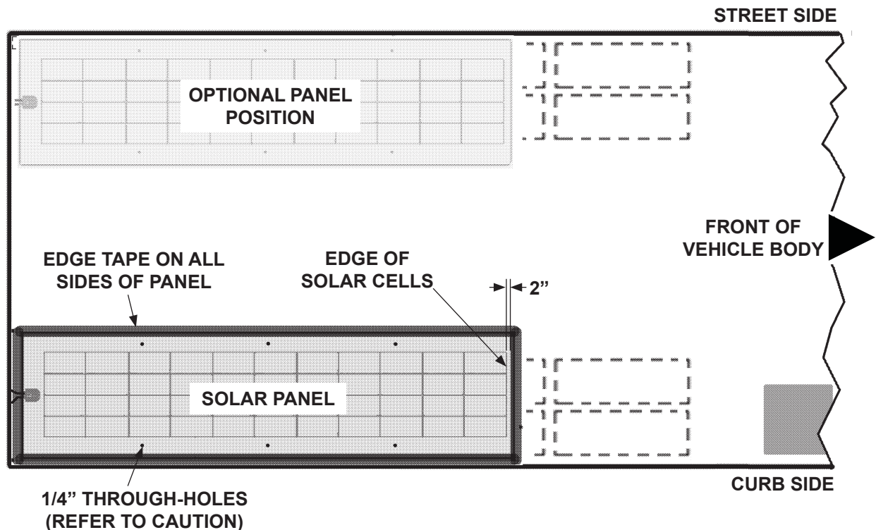
APPLYING EDGE TAPE TO SOLAR PANEL (PANEL SHOWN POSITIONED FOR MOUNTING WITH MECHANICAL FASTENERS)
