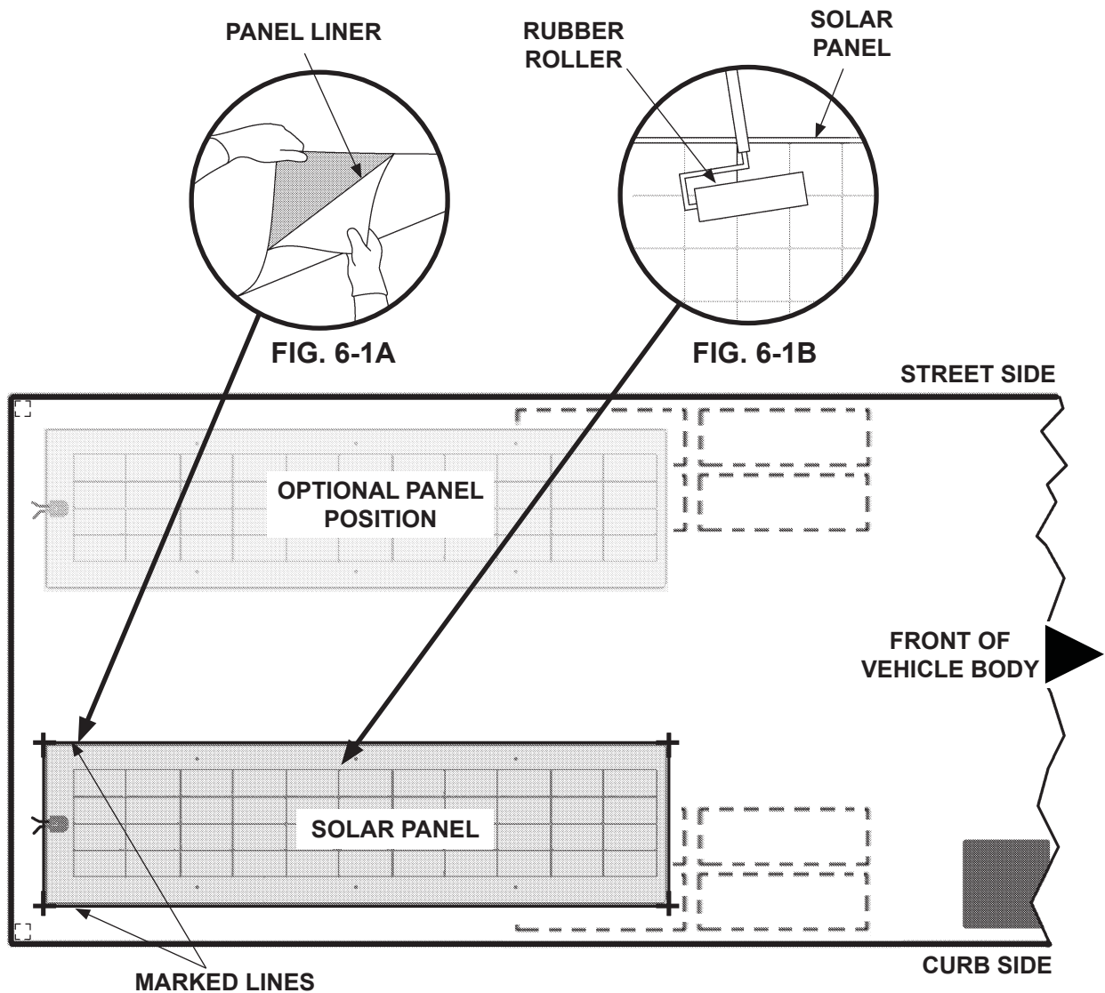
ATTACHING SOLAR PANEL FIG. 6-1
