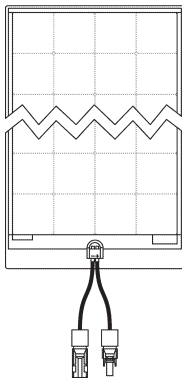
4 X 11 SOLAR PANEL WITH JBOX CABLES, 110W P/N 211626-01 QTY. 1
