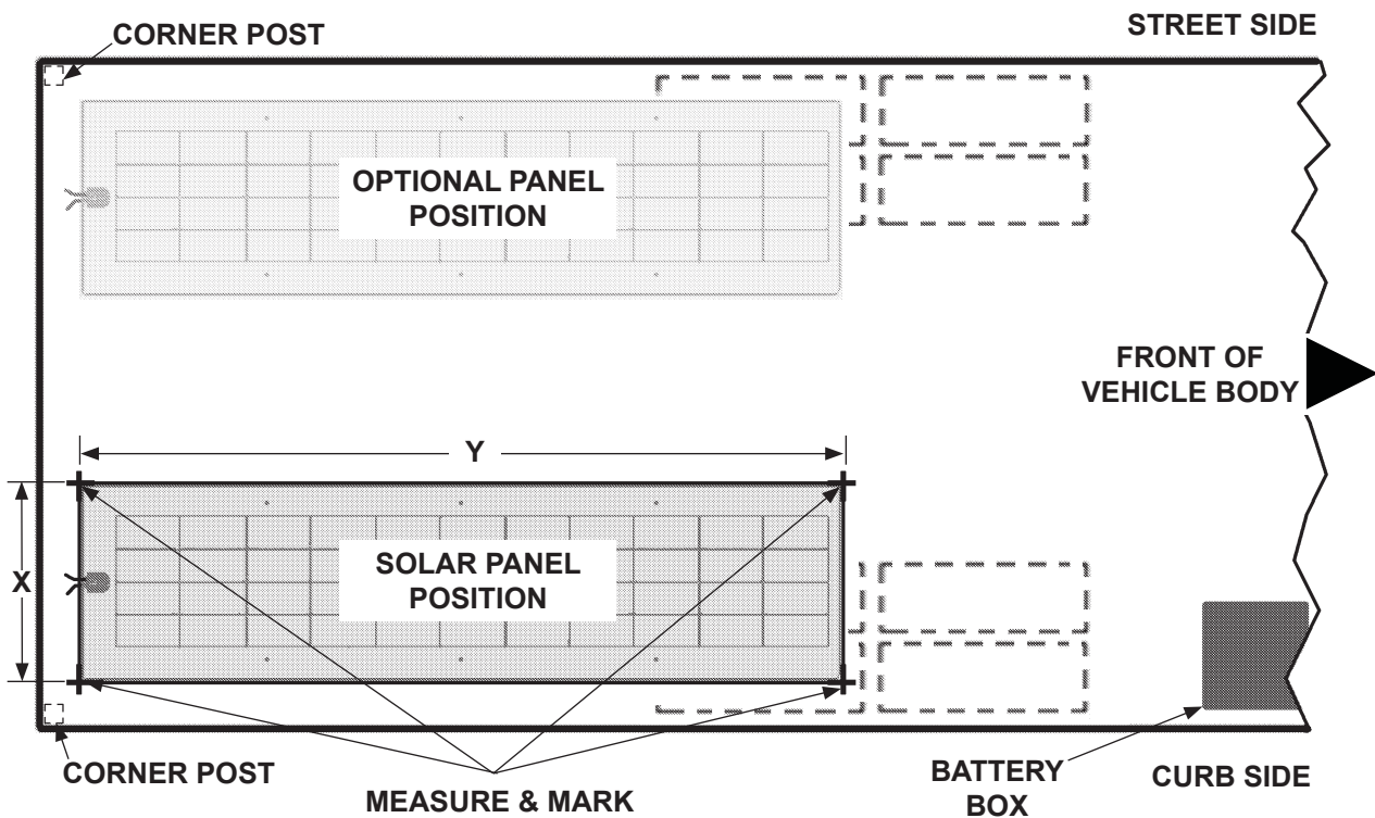
MARKING POSITION OF SOLAR PANEL ON ROOF OF TRUCK/TRAILER FIG. 5-1
