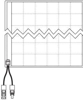
6 X 12 SOLAR PANEL WITH JBOX CABLES, 360W P/N 211629-01 QTY. 1
