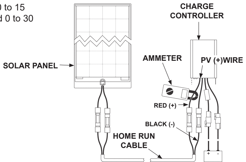
MEASURING CURRENT ON PV (+) WIRE FIG. 15-1
