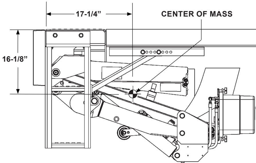
GPTWR-25 & GPTWR-3 CENTER OF MASS (STOWED POSITION) FIG. 13-1
