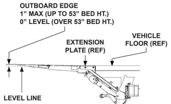
PLATFORM EDGE ABOVE BED LEVEL FIG. 53-3
