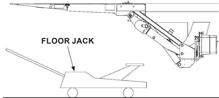
REMOVING JACK FIG. 44-1
