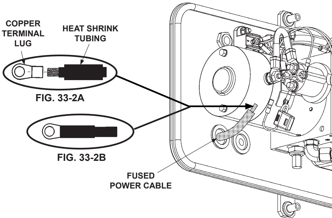
TYPICAL FUSED POWER CABLE ROUTING FIG. 33-2
