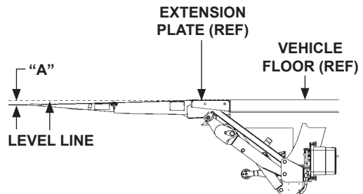
PLATFORM EDGE BELOW BED LEVEL FIG. 52-2
