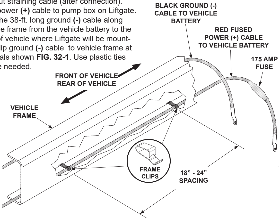
RUNNING POWER & GROUND CABLES TO TAIL LIFT ON TRUCK FIG. 32-1
