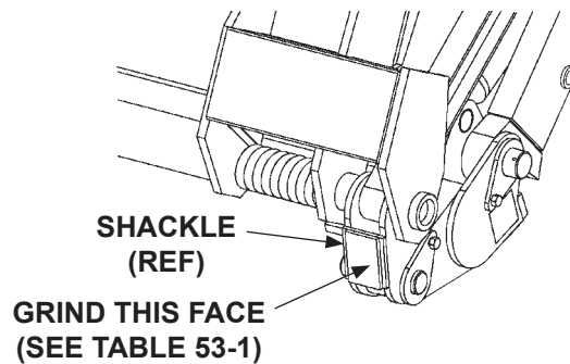
GRINDING PLATFORM STOPS (CURBSIDE SHOWN) FIG. 53-2
