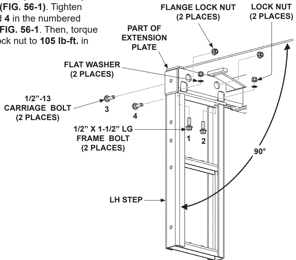
BOLTING STEP TO EXTENSION PLATE (LH DUAL STEP SHOWN) FIG. 56-1
