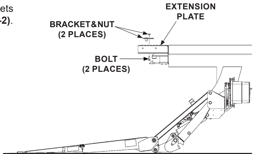
REMOVING INSTALLATION BRACKETS FIG. 45-2
