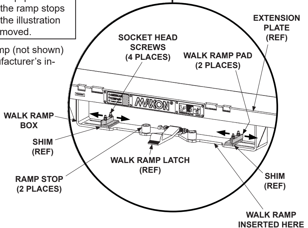
ADJUSTING WALK RAMP PADS FIG. 59-1A
