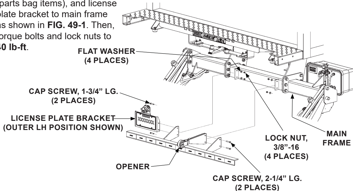
BOLTING ON ICC BUMPER, OPENER & LICENSE PLATE BRACKET FIG. 49-1
