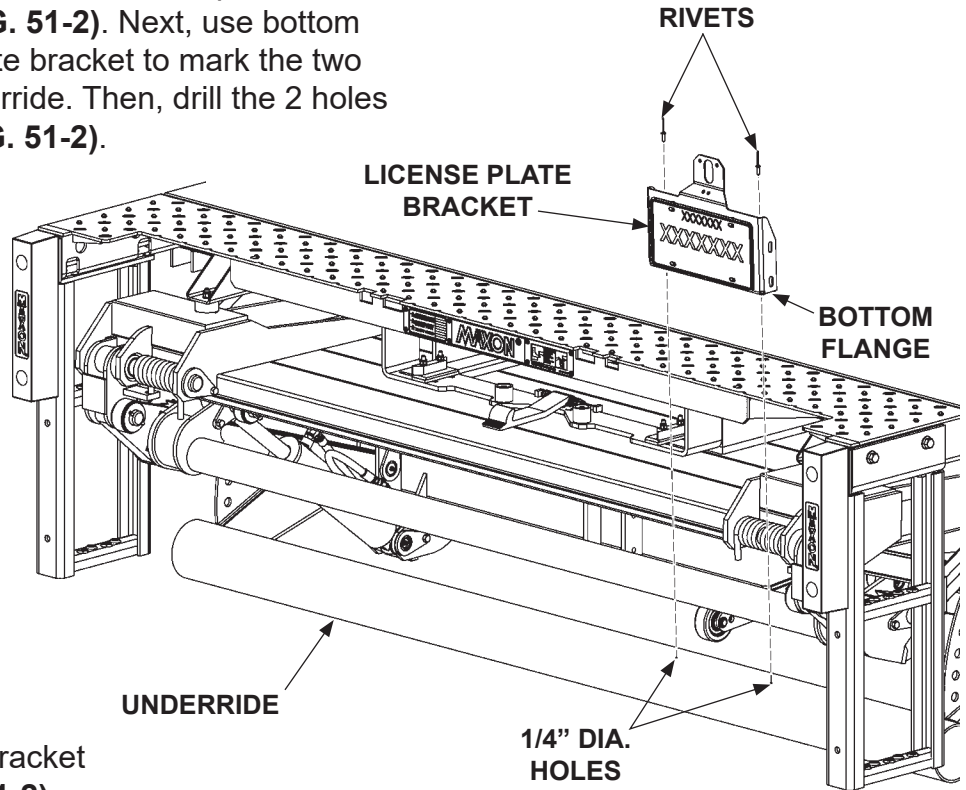
EXAMPLE FOR POSITIONING & RIVETING LICENSE PLATE BRACKET TO UNDERRIDE FIG. 51-2
