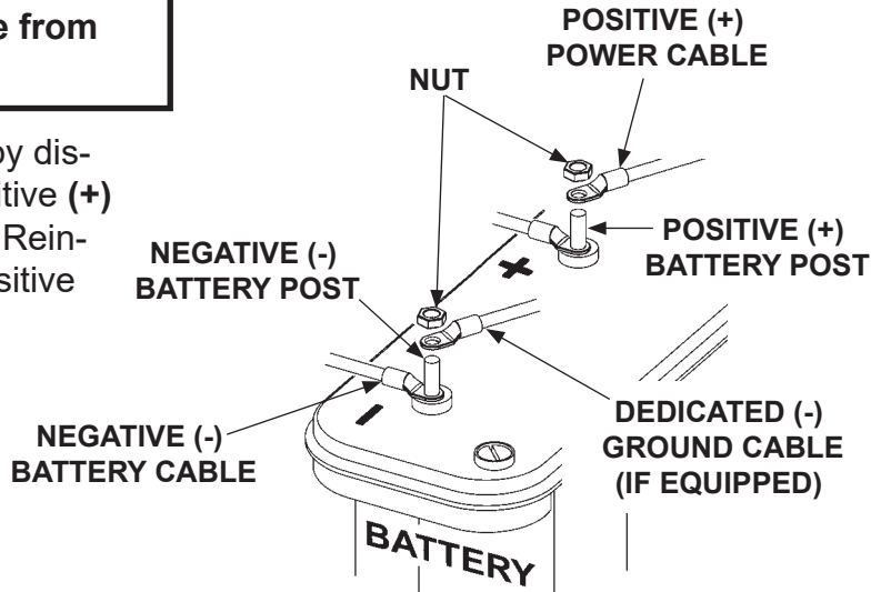
DISCONNECTING BATTERY POWER FIG. 50-1
