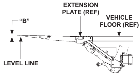
PLATFORM EDGE ABOVE BED LEVEL FIG. 53-1
