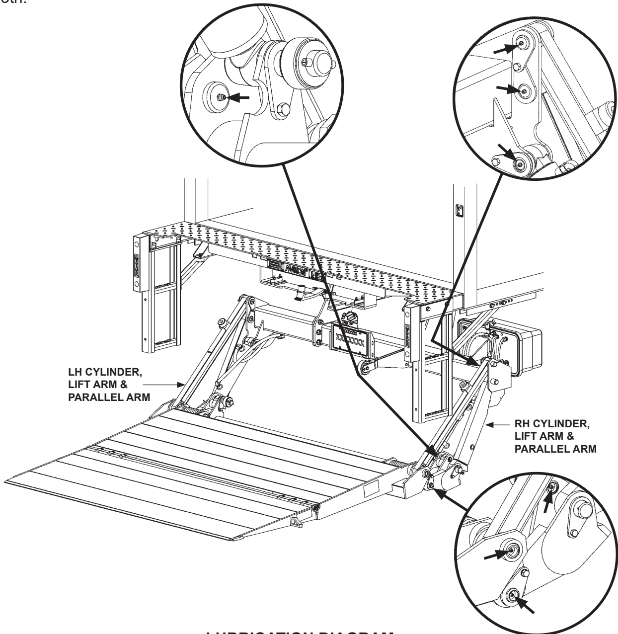
LUBRICATION DIAGRAM FIG. 61-1
