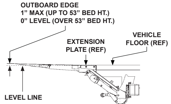
PLATFORM EDGE AT OR ABOVE BED LEVEL FIG. 52-1
