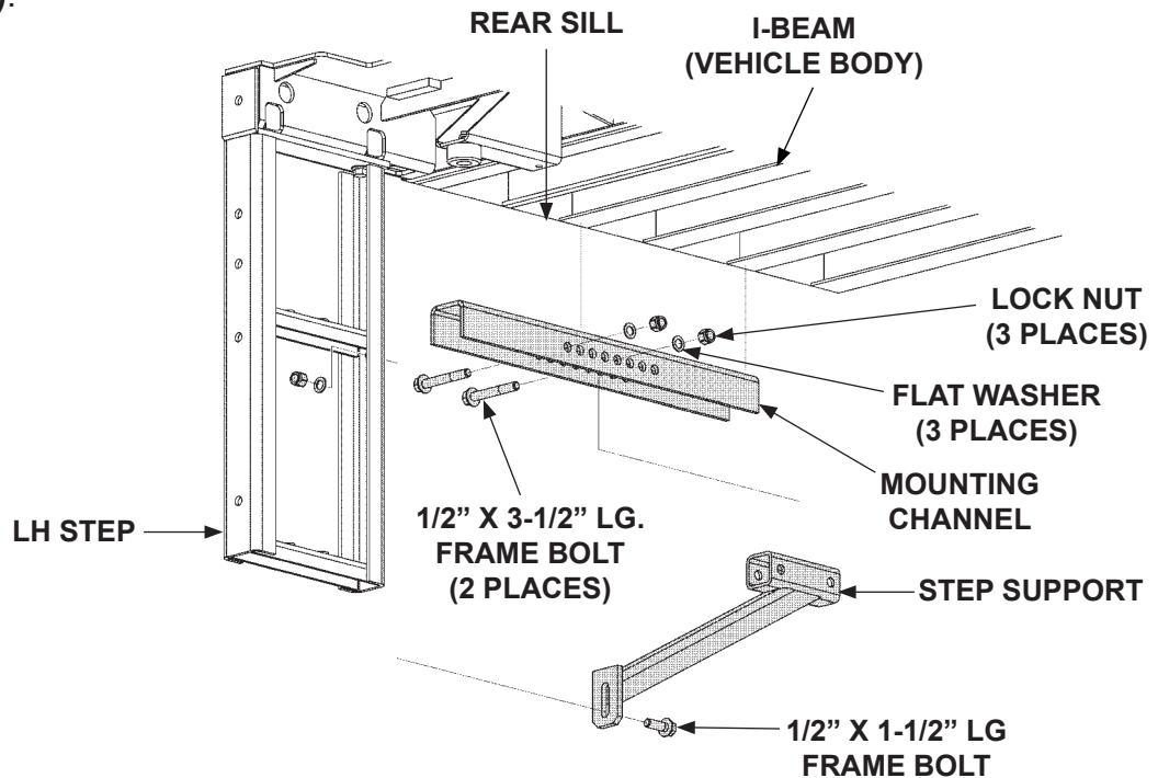
BOLTING SUPPORT TO MOUNTING CHANNEL & STEP (LH STEP & SUPPORT SHOWN) FIG. 57-1
