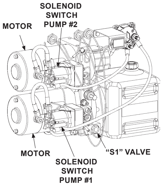
DUAL PUMP POWER UNIT FIG. 67-1
