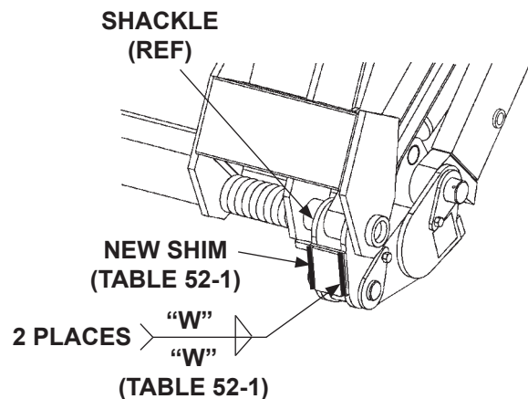
WELDING SHIMS (CURBSIDE SHOWN) FIG. 52-3
