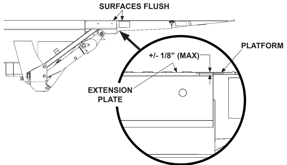
DIFFERENCE IN HEIGHT FOR TOP OF PLATFORM & EXTENSION PLATE (LH VIEW) FIG. 47-2
