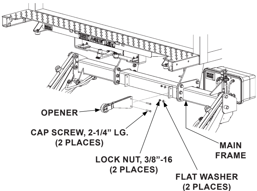
BOLTING ON OPENER & LICENSE PLATE BRACKET FIG. 50-2
