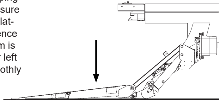
LOWERING PLATFORM FIG. 44-2
