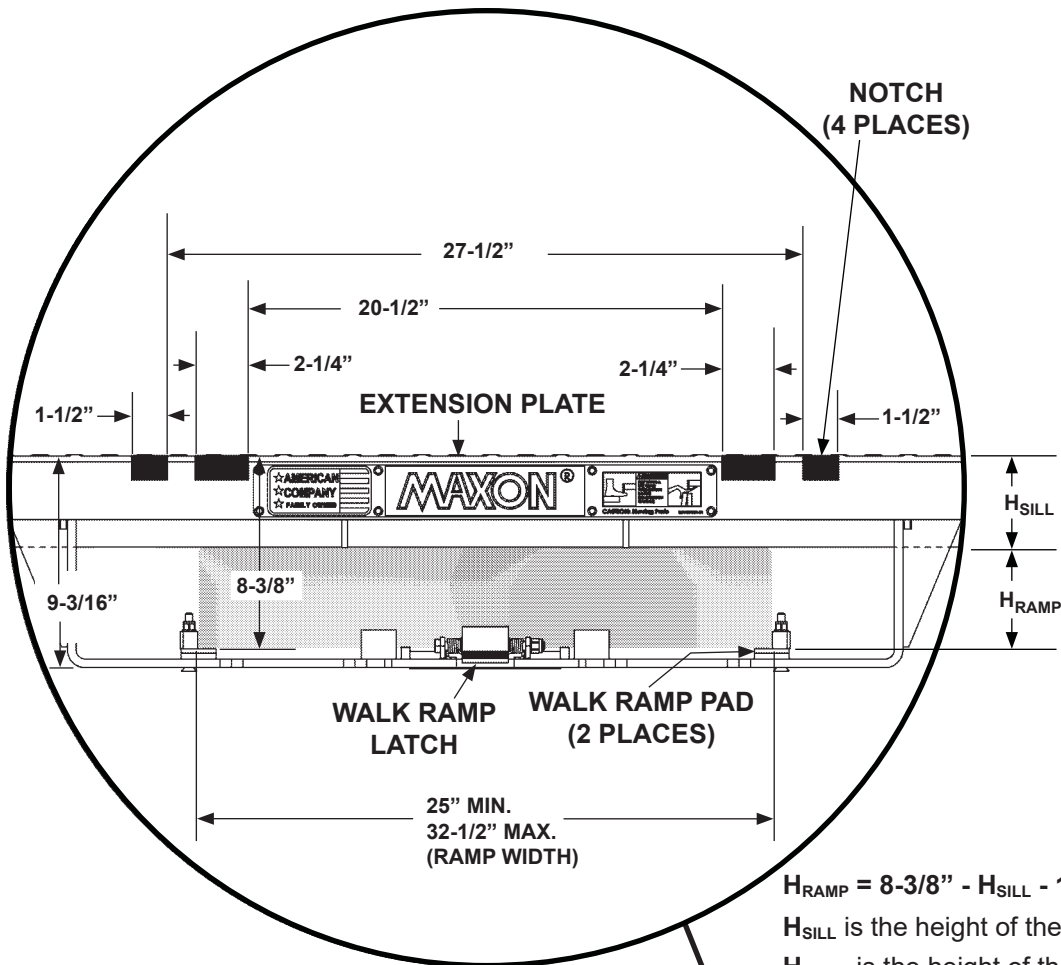
WALK RAMP BOX CLEARANCE DIMENSIONS (FOR REFERENCE ONLY) FIG. 11-1A
