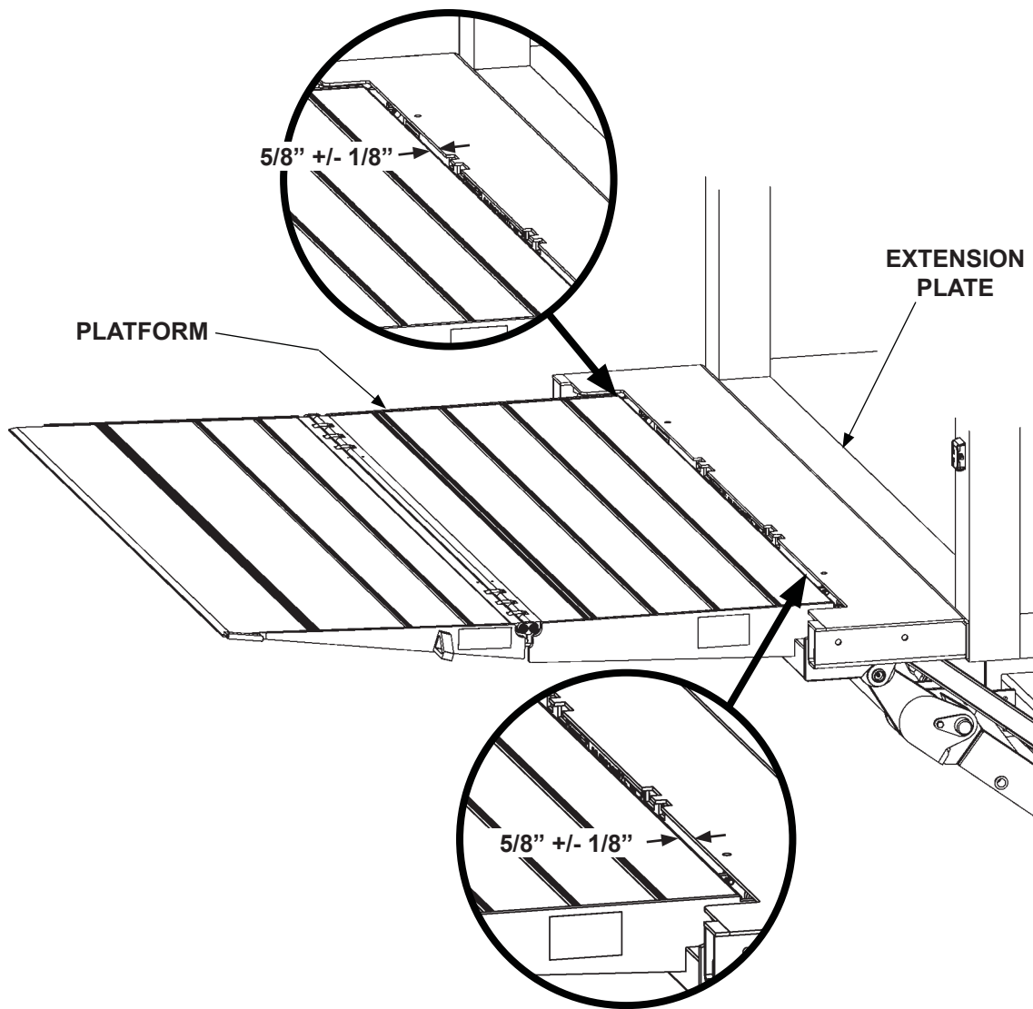
CHECKING GAP BETWEEN PLATFORM AND EXTENSION PLATE FIG. 46-1
