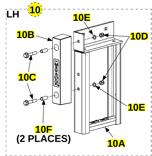
SINGLE STEP ASSEMBLY WITH RUBBER BUMPER
