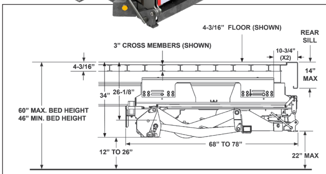
Clearances For GPSLRT With 68" To 78" Slide Rails (Truck)
