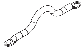
BLACK CABLE ASSEMBLY, 2 GA, 8" LG. P/N 251871-14 QTY. 1
