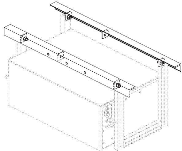
REMOTE BATTERY BOX MOUNTING KIT P/N 287585-02 (4- BATTERY BOX SHOWN) QTY. 1
