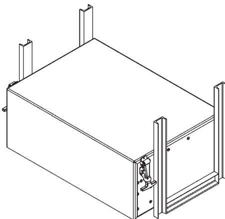
4-BATTERY BOX ASSEMBLY P/N 289690-11, 289690-12, 289690-13 QTY. 1
