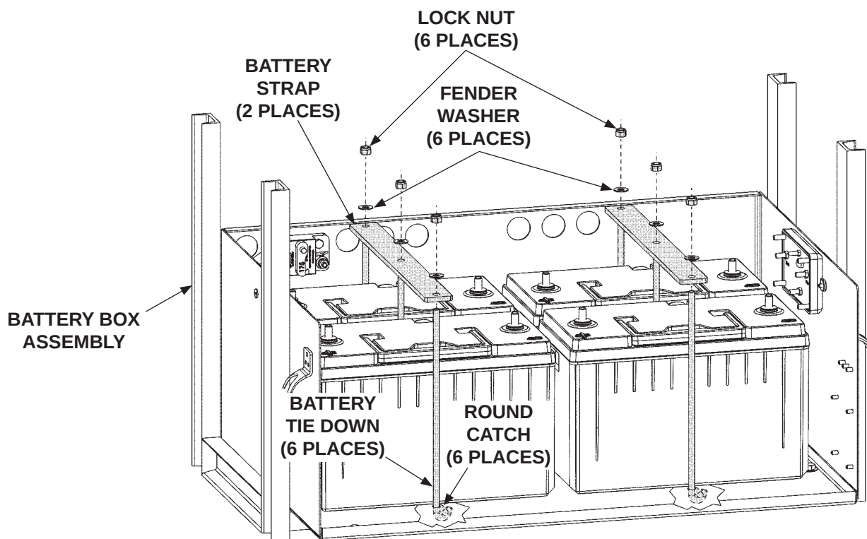
SECURING BATTERIES (4-BATTERY BOX) FIG. 15-2
