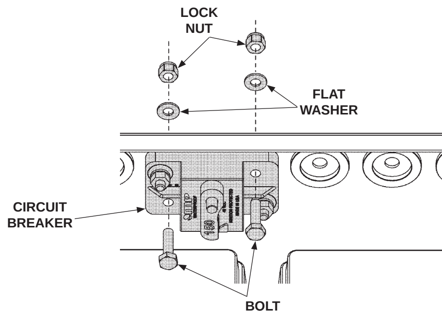
MOUNTING CIRCUIT BREAKER (4-BATTERY BOX) FIG. 16-2
