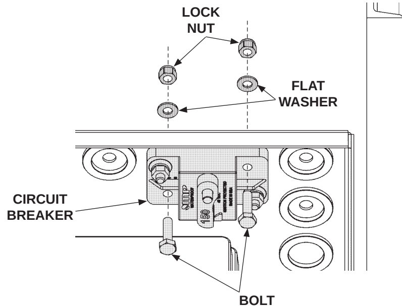
MOUNTING CIRCUIT BREAKER (2-BATTERY BOX) FIG. 16-1
