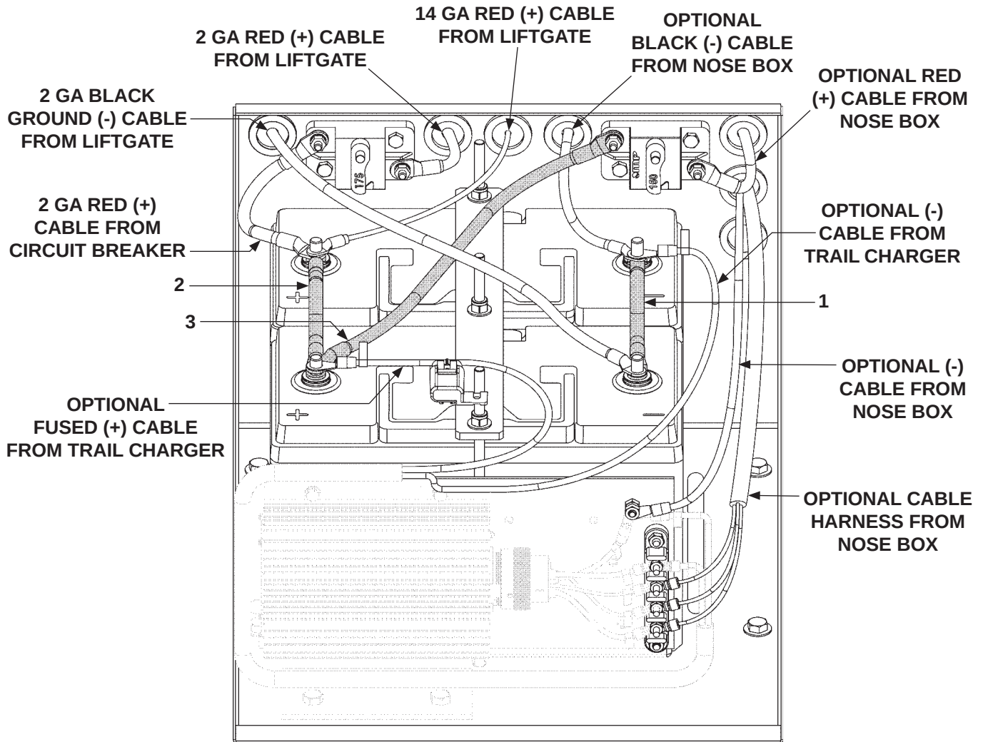
12 VOLT BATTERY CONNECTIONS (2-BATTERY BOX) FIG. 20-1
