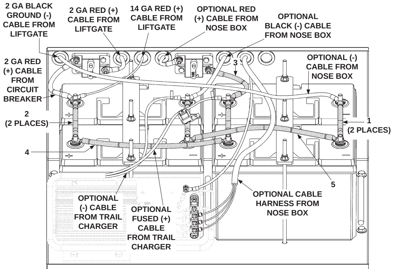
12 VOLT BATTERY CONNECTIONS (4-BATTERY BOX) FIG. 21-1
