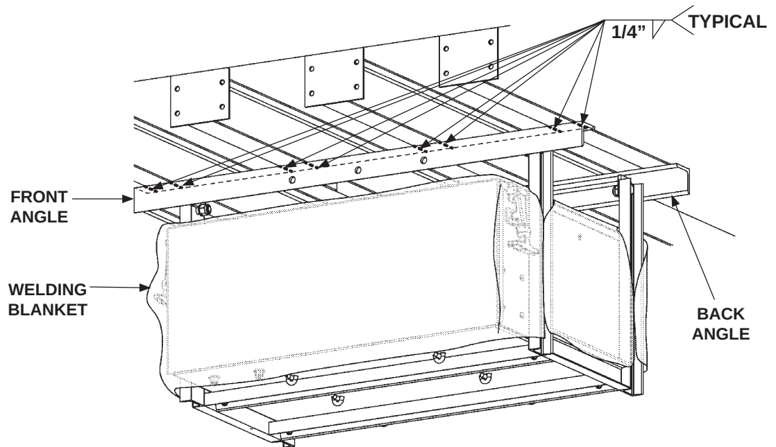
WELDING BATTERY BOX ASSEMBLY (4-BATTERY BOX SHOWN) FIG. 14-1
