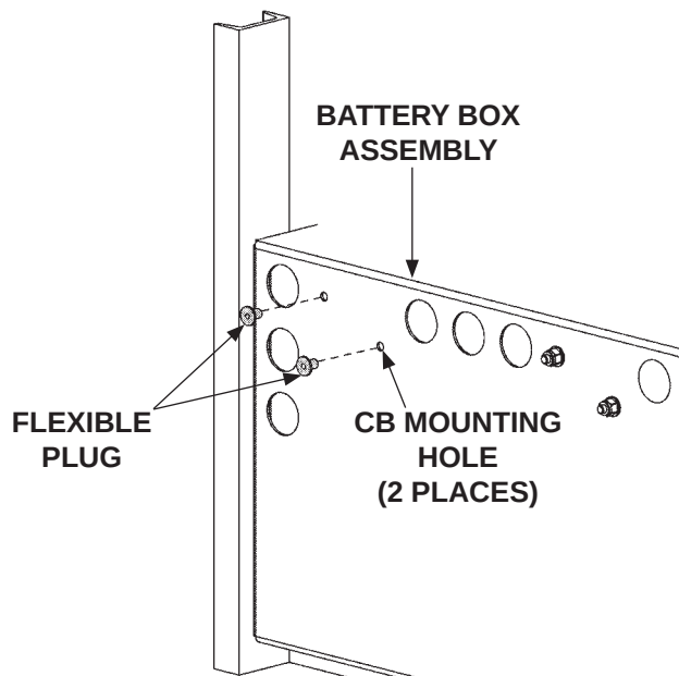
PLUGGING CB MOUNTING HOLES (2-BATTERY BOX) FIG. 11-1
