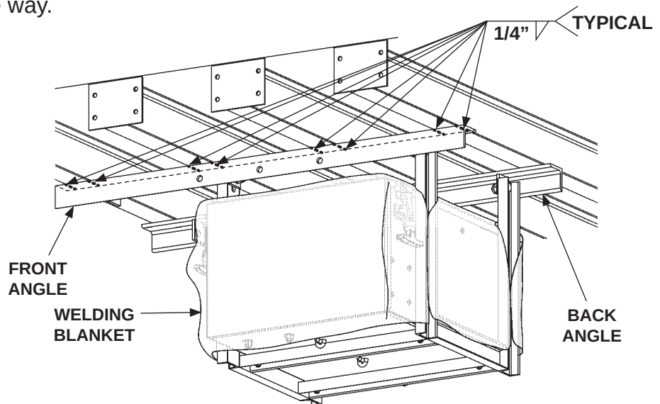
WELDING BATTERY BOX ASSEMBLY (2-BATTERY BOX SHOWN) FIG. 13-1
