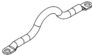
RED CABLE ASSEMBLY, 2 GA, 8" LG. P/N 269308-10 QTY. 1
