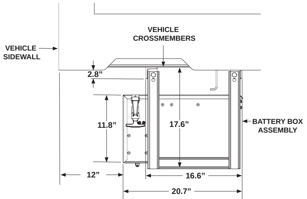
BATTERY BOX ASSEMBLY CLEARANCE DIMENSIONS FIG. 12-2
