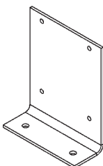
GALVANIZED BRACKET, TRAIL CHARGER P/N 289722-01G (KITS 289690-01 & 289690-03) QTY. 1
