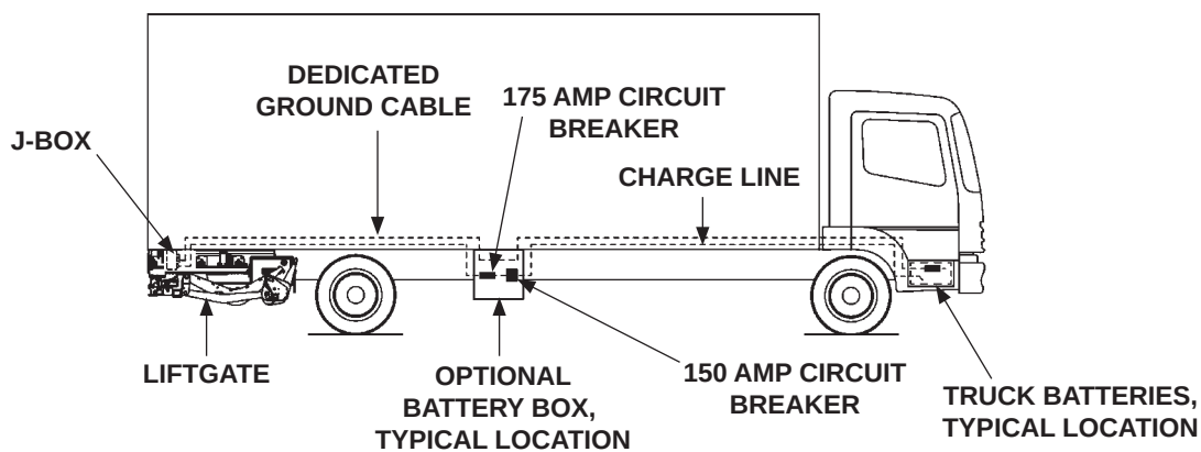
OPTIONAL BATTERY BOX INSTALLED ON TRUCK (GPSLR SHOWN) FIG. 8-2
