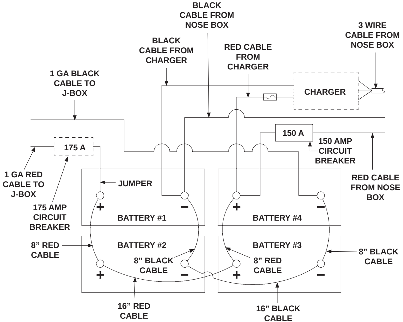
BATTERY CONNECTIONS - 4-BATTERY BOX (WITH DIRECT CHARGING AND CHARGER) FIG. 25-1
