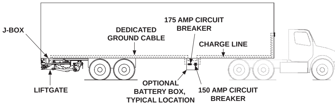
OPTIONAL BATTERY BOX INSTALLED ON TRAILER (GPSLR SHOWN) FIG. 8-1
