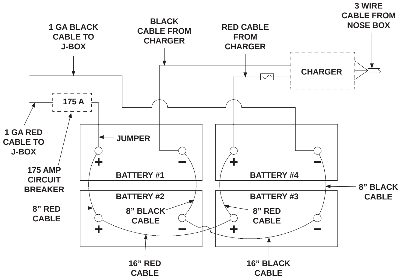
BATTERY CONNECTIONS - 4-BATTERY BOX (WITH CHARGER) FIG. 27-1
