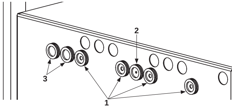
GROMMET LOCATIONS FOR KIT P/N 289690-12 FIG. 19-2
