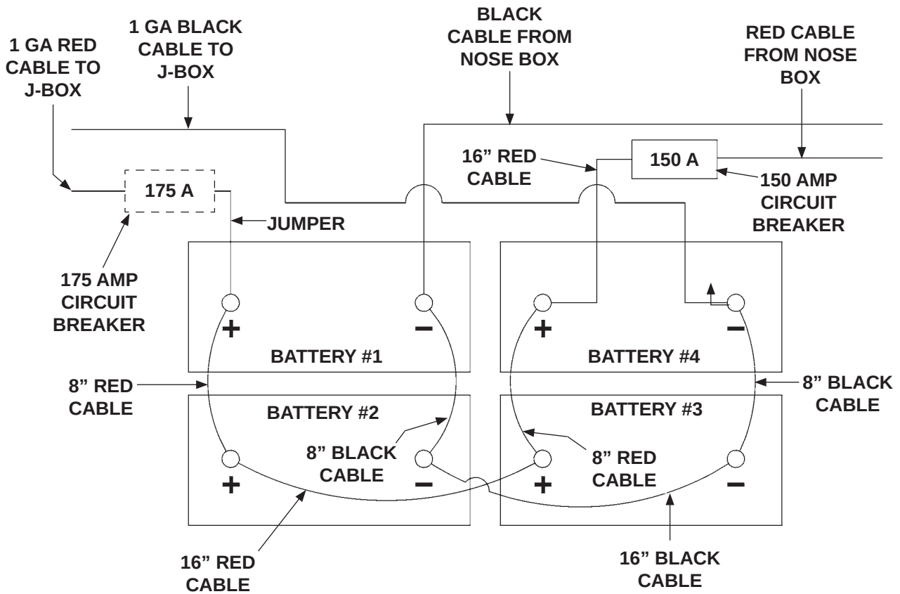
BATTERY CONNECTIONS - 4-BATTERY BOX (WITH DIRECT CHARGING) FIG. 26-1
