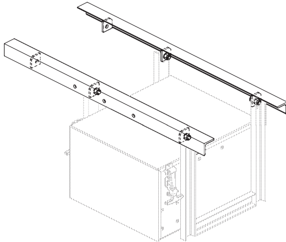
REMOTE BATTERY BOX MOUNTING KIT P/N 287585-02 (2- BATTERY BOX SHOWN) QTY. 1
