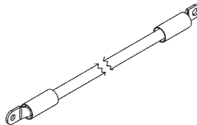
RED CABLE ASSEMBLY, 2 GA, 16" LG. P/N 269308-16 (KITS 289690-01 & 289690-02) QTY. 1
