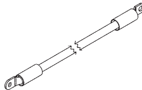
RED CABLE ASSEMBLY, 2 GA, 16" LG. P/N 269308-16 (KITS 289690-11 & 289690-12) QTY. 1
