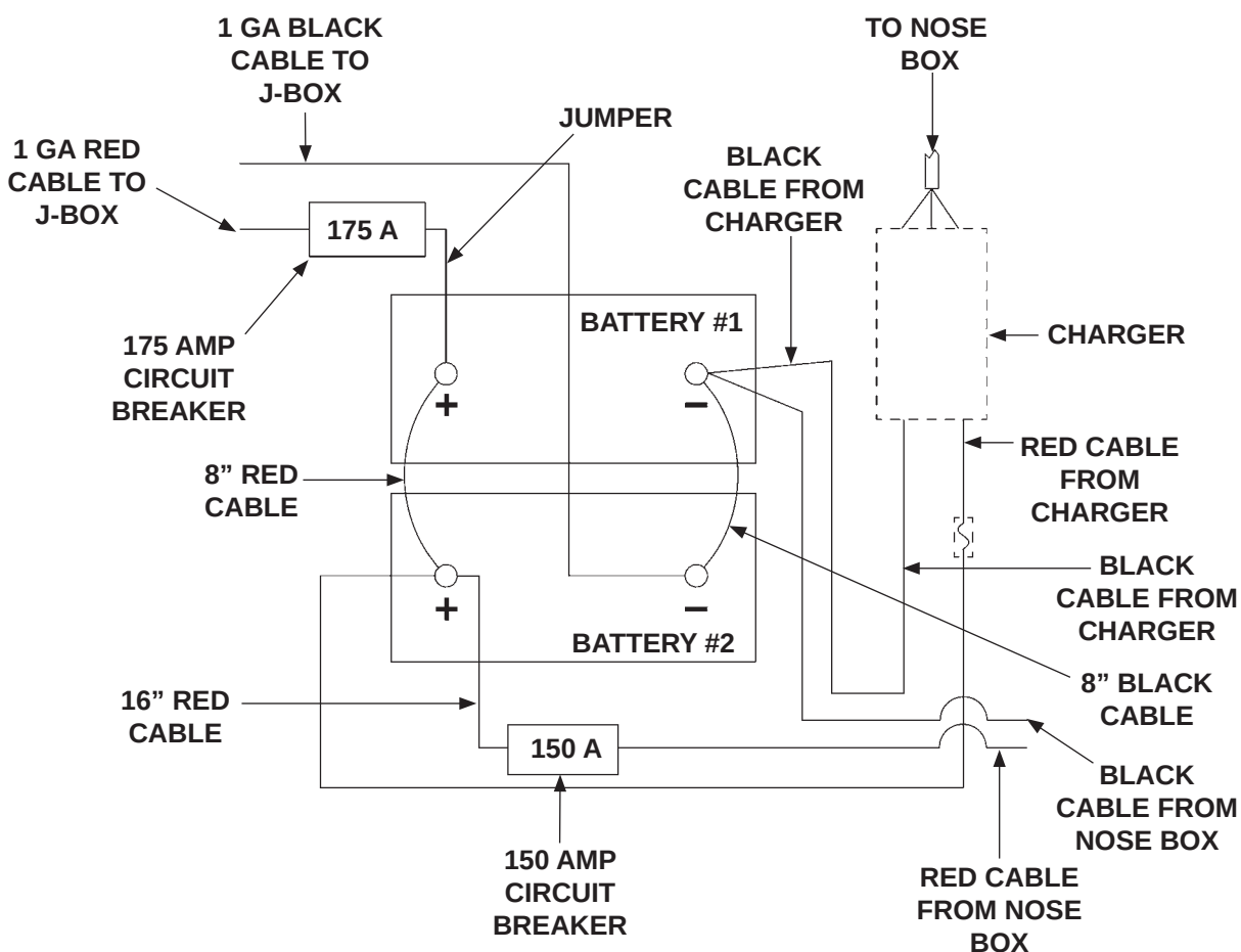
BATTERY CONNECTIONS - 2-BATTERY BOX (WITH DIRECT CHARGING AND CHARGER) FIG. 22-1
