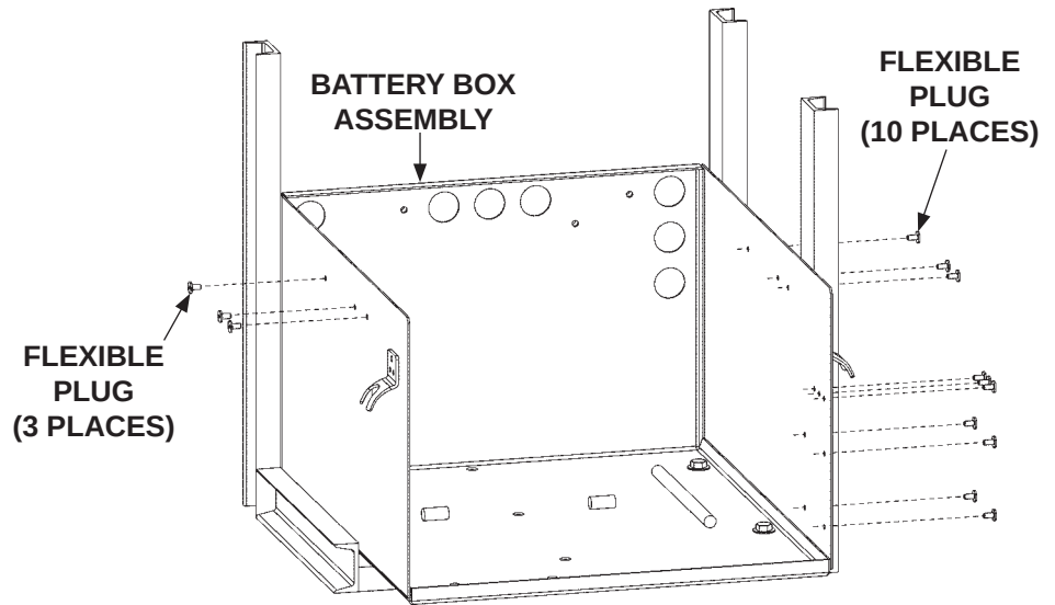
INSTALLING FLEXIBLE PLUGS (2-BATTERY BOX) FIG. 10-1
