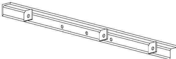
ANGLE WELDMENT, BATTERY BOX, REMOTE MOUNT, FRONT P/N 289538-01 QTY. 1
