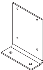
GALVANIZED BRACKET, TRAIL CHARGER P/N 289722-01G (KITS 289690-11 & 289690-13) QTY. 1
