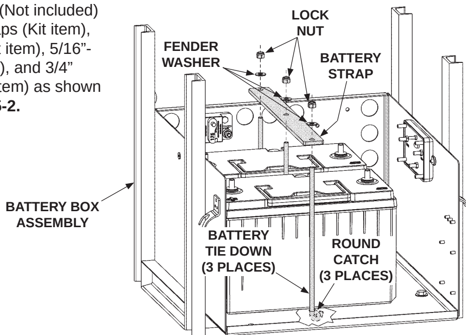
SECURING BATTERIES (2-BATTERY BOX) FIG. 15-1
