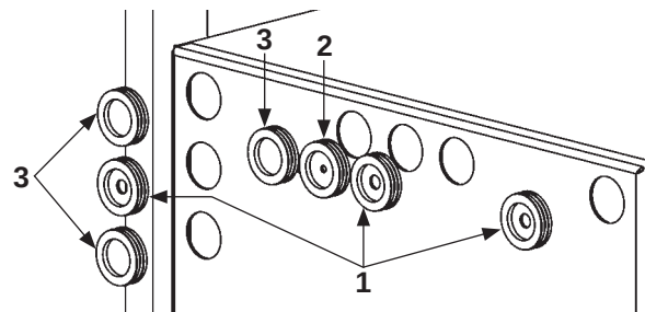
GROMMET LOCATIONS FOR KIT P/N 289690-03 FIG. 18-3
