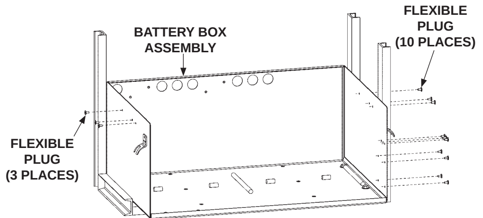
INSTALLING FLEXIBLE PLUGS (4-BATTERY BOX) FIG. 10-2
