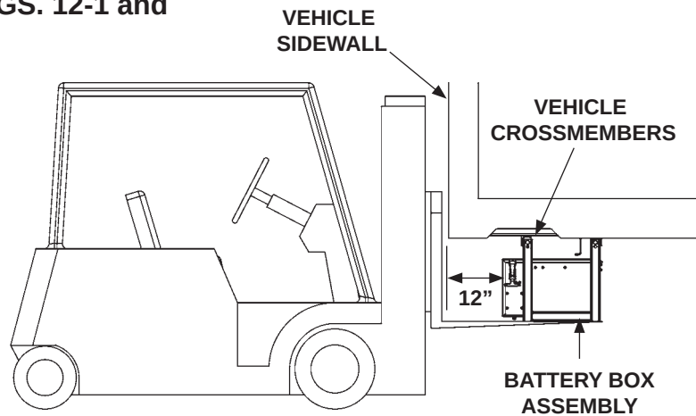
POSITIONING BATTERY BOX ASSEMBLY FIG. 12-1
