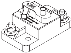
150 AMP CIRCUIT BREAKER P/N 907207-02 (KITS 289690-11 & 289690-12) QTY. 1
