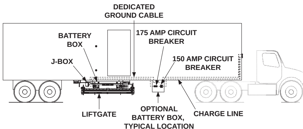
OPTIONAL BATTERY BOX INSTALLED ON TRAILER (RA SHOWN) FIG. 9-1
