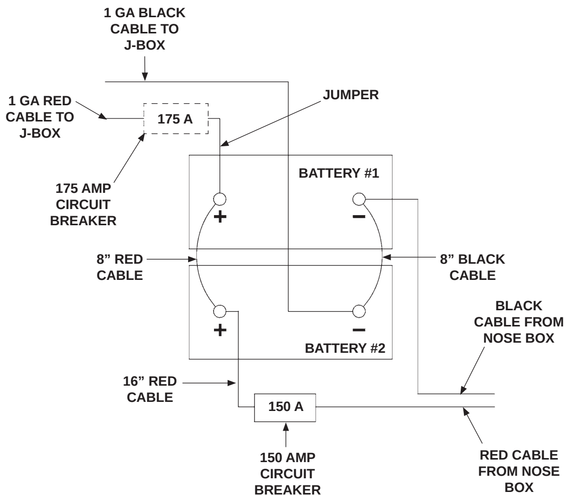
BATTERY CONNECTIONS - 2-BATTERY BOX (DIRECT CHARGING) FIG. 23-1
