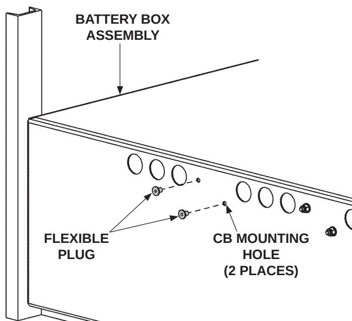
PLUGGING CB MOUNTING HOLES (4-BATTERY BOX) FIG. 11-2
