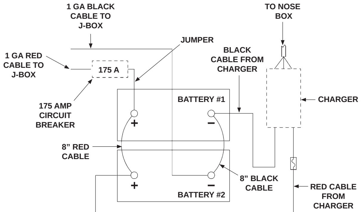
BATTERY CONNECTIONS - 2-BATTERY BOX (WITH CHARGER, NO DIRECT CHARGING) FIG. 24-1
