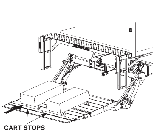
LOADING PLATFORM AT GROUND LEVEL (CART STOPS CLOSED) FIG. 27-1
