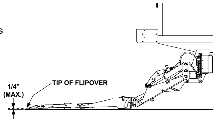
PLATFORM & SHACKLES TOUCH GROUND FIG. 59-2
