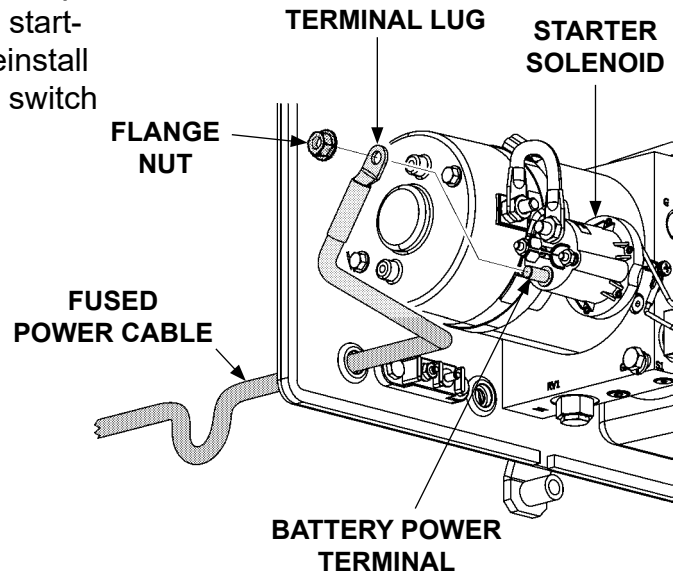
CONNECTING FUSED POWER CABLE (GRAVITY DOWN PUMP SHOWN) FIG. 37-1
