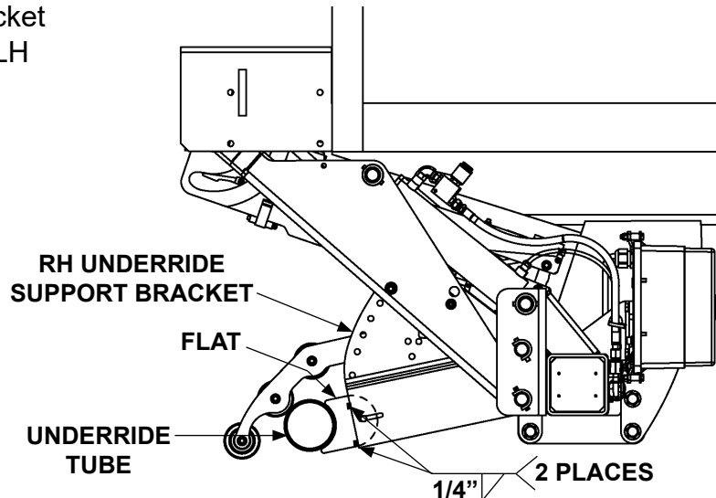
TACK WELDING FLATS TO SUPPORT BRACKETS (RH SIDE SHOWN) FIG. 72-1
