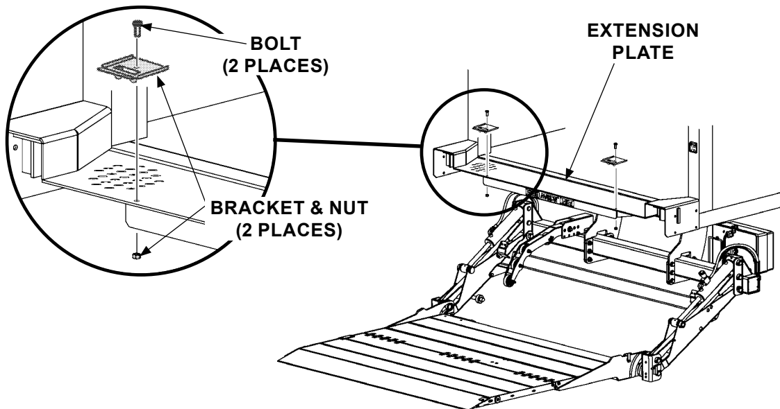
REMOVING LOCKING BRACKETS FIG. 46-1
