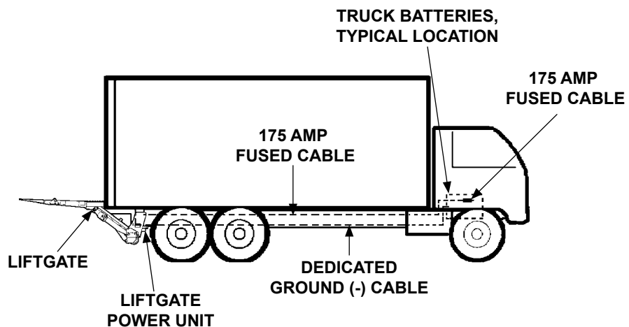
RECOMMENDED LIFTGATE & POWER CABLE INSTALLATION ON TRUCK
