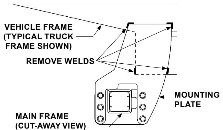
REMOVING WELDS FROM MOUNTING PLATE (RH SIDE SHOWN) FIG. 56-2
