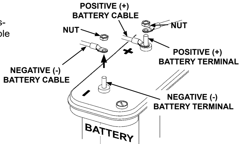
DISCONNECTING (-) BATTERY CABLE FIG. 44-1
