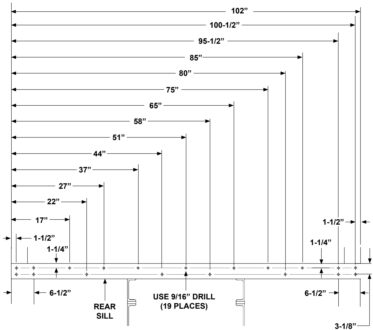
REAR SILL - HOLE LOCATIONS FOR 102" WIDE VEHICLE FIG. 17-1
