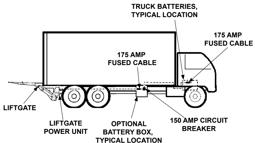
RECOMMENDED LIFTGATE & BATTERY BOX INSTALLATION ON TRUCK FIG. 26-2
