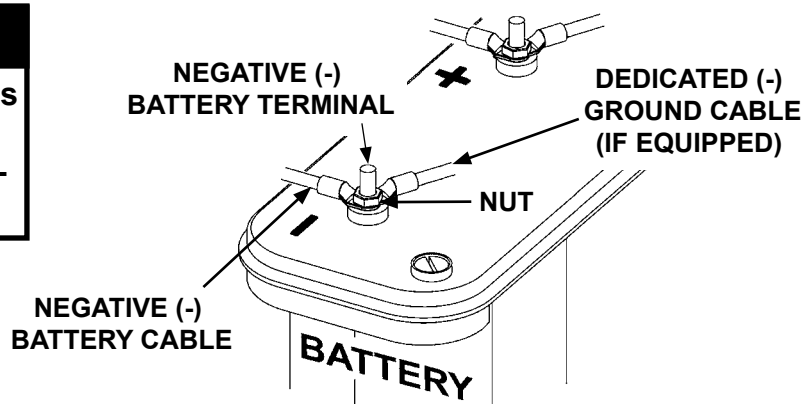
RECONNECTED BATTERY CABLES FIG. 44-3
