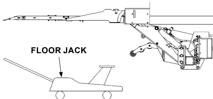
REMOVING JACK FIG. 58-1
