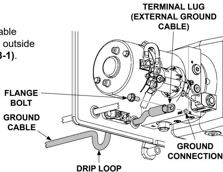
BOLTING GROUND CABLE TO PUMP FIG. 38-2
