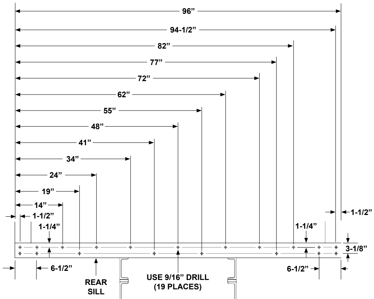
REAR SILL - HOLE LOCATIONS FOR 96" WIDE VEHICLE
