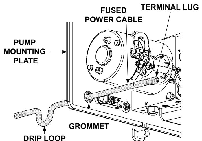
ROUTING FUSED POWER CABLE FIG. 36-4
