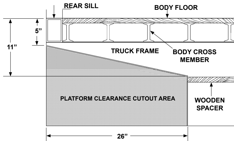
VEHICLE FRAME CUT FOR ALL GPTLR MODELS FIG. 13-1
