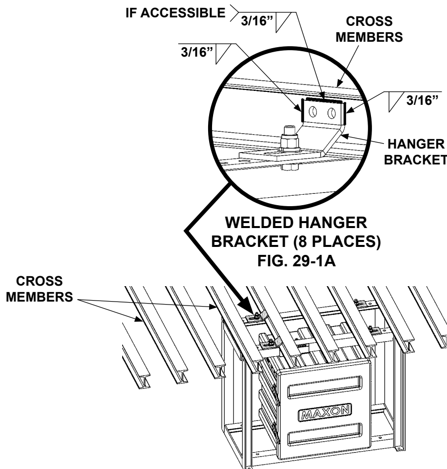
HANGER BRACKETS WELDED TO VEHICLE CROSS MEMBERS FIG. 29-1
