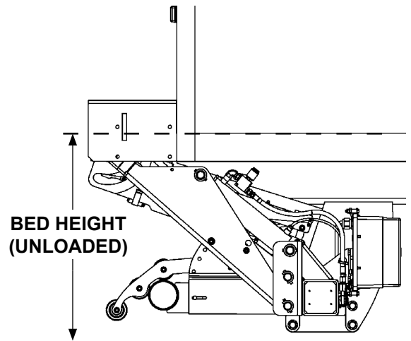
MEASURING BED HEIGHT (STANDARD UNDERRIDE SHOWN) FIG. 66-2
