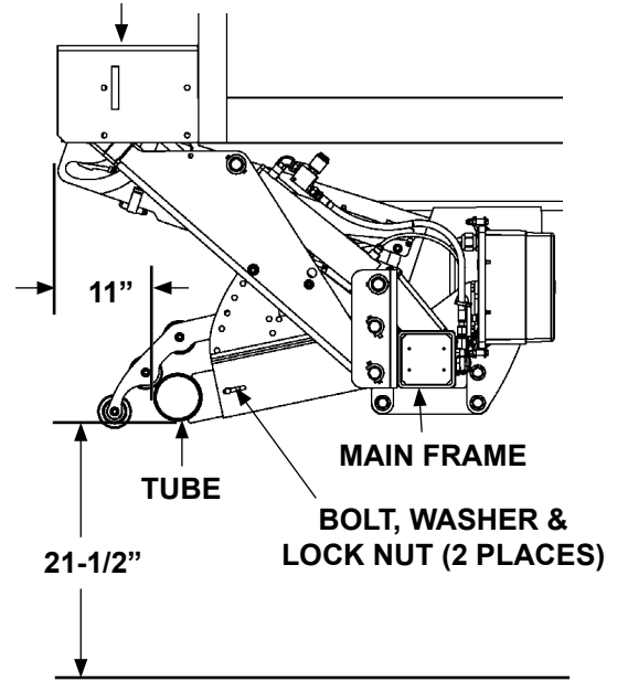
UNDERRIDE TUBE ADJUSTMENT (RH SIDE SHOWN) FIG. 71-1
