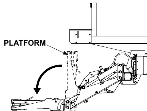
UNFOLDING PLATFORM FIG. 62-2
