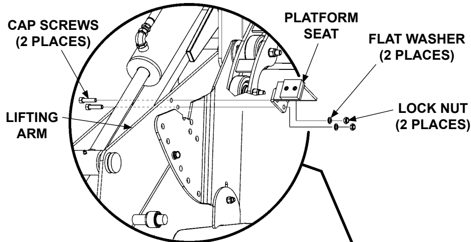
BOLTING ON PLATFORM SEAT (LH SEAT SHOWN) FIG. 77-1A
