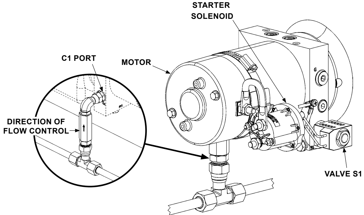
GRAVITY DOWN POWER UNIT FIG. 84-1
