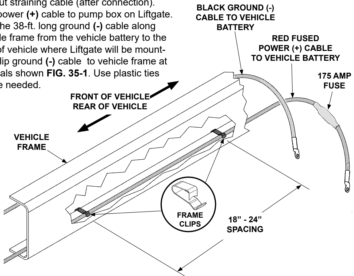
RUNNING POWER & GROUND CABLES TO LIFTGATE ON TRUCK
