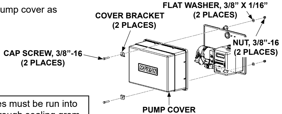
UNBOLTING PUMP COVER FIG. 36-1
