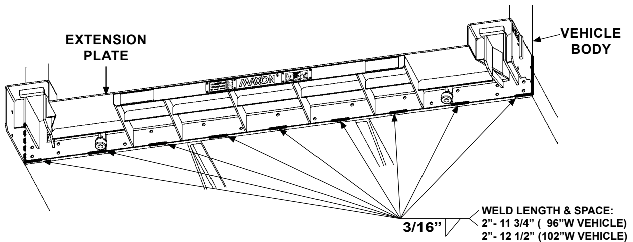
EXTENSION PLATE WELDS - VIEWED FROM UNDERNEATH FIG. 20-1
