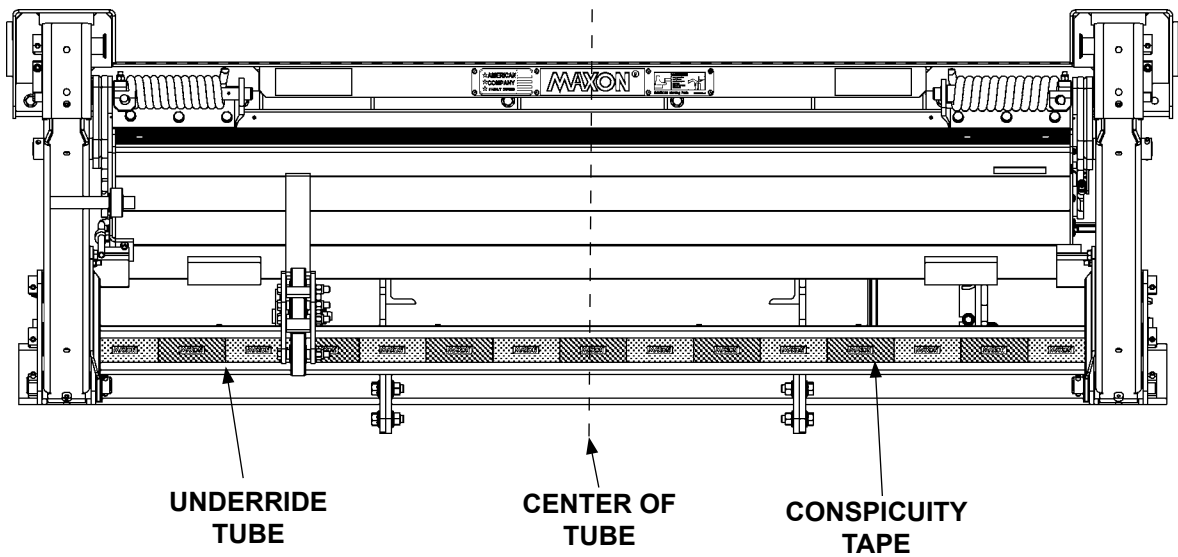
ATTACH CONSPICUITY TAPE FIG. 78-1
