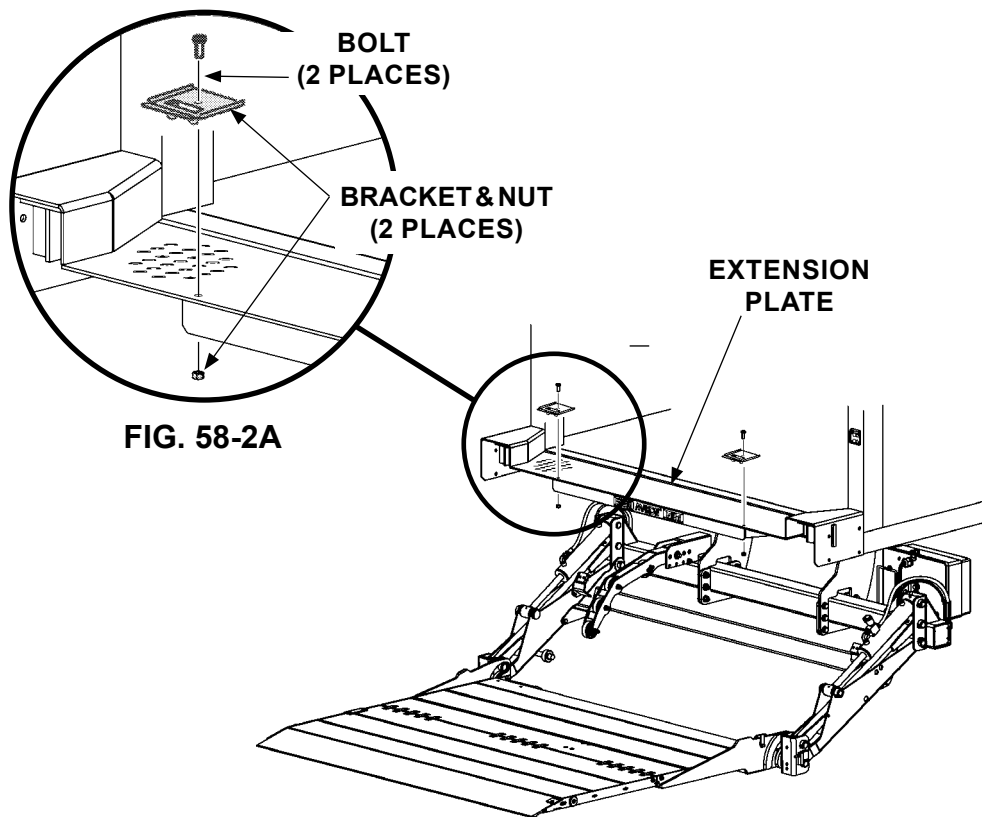
REMOVING INSTALLATION BRACKETS FIG. 58-2
