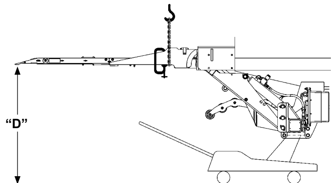
LIFTGATE CLEARANCE DIMENSIONS FIG. 56-3
