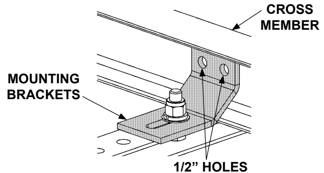
MARK AND DRILL BRACKET HOLES FIG. 28-1
