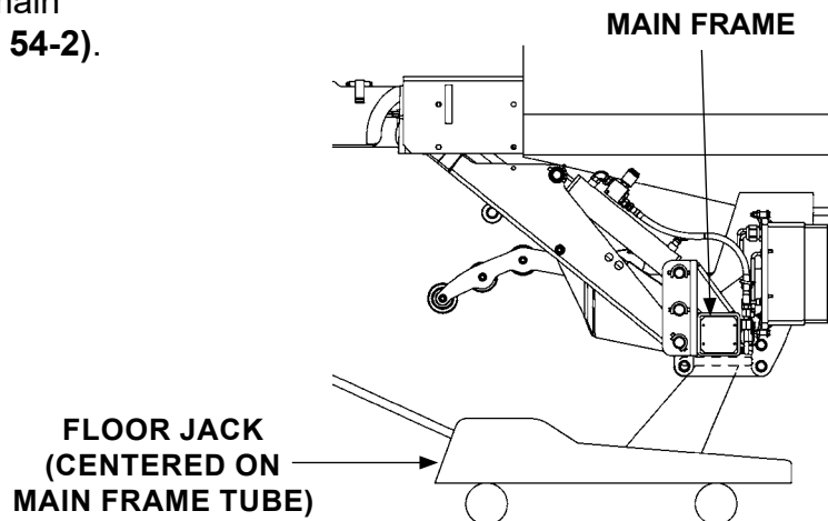
SUPPORTING LIFTGATE FIG. 54-2
