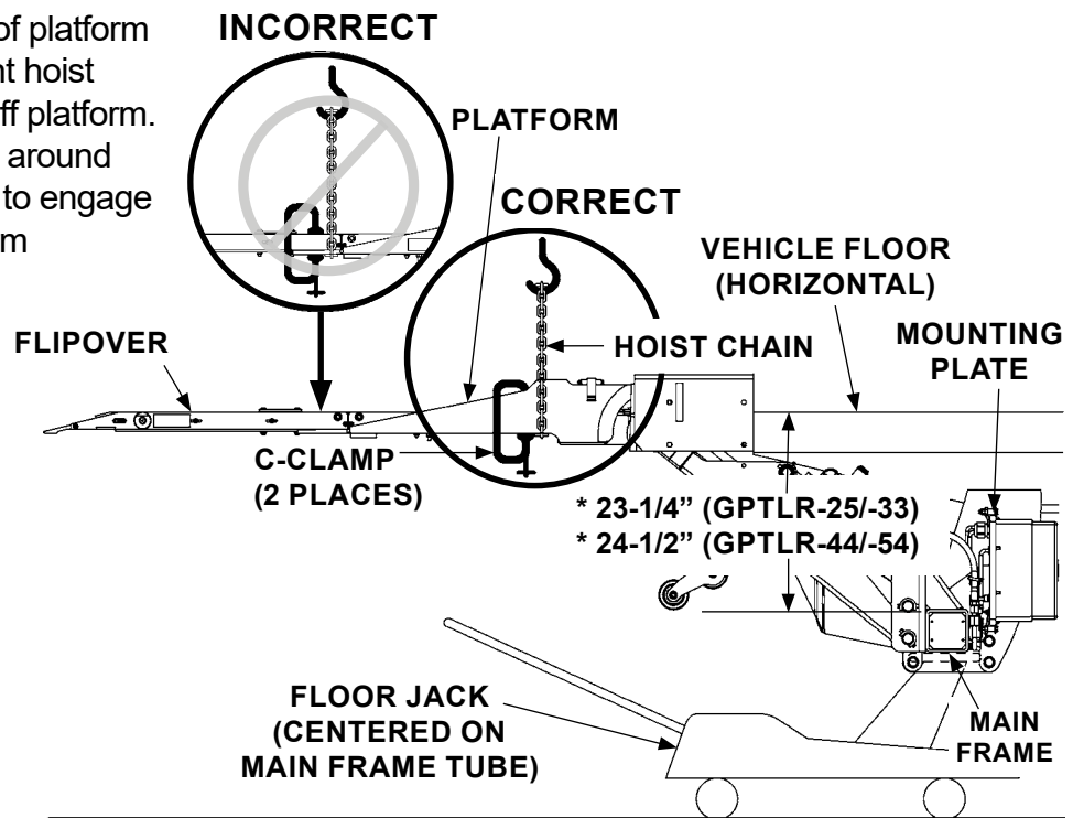
CORRECT WAY TO HOIST LIFTGATE FIG. 55-1
