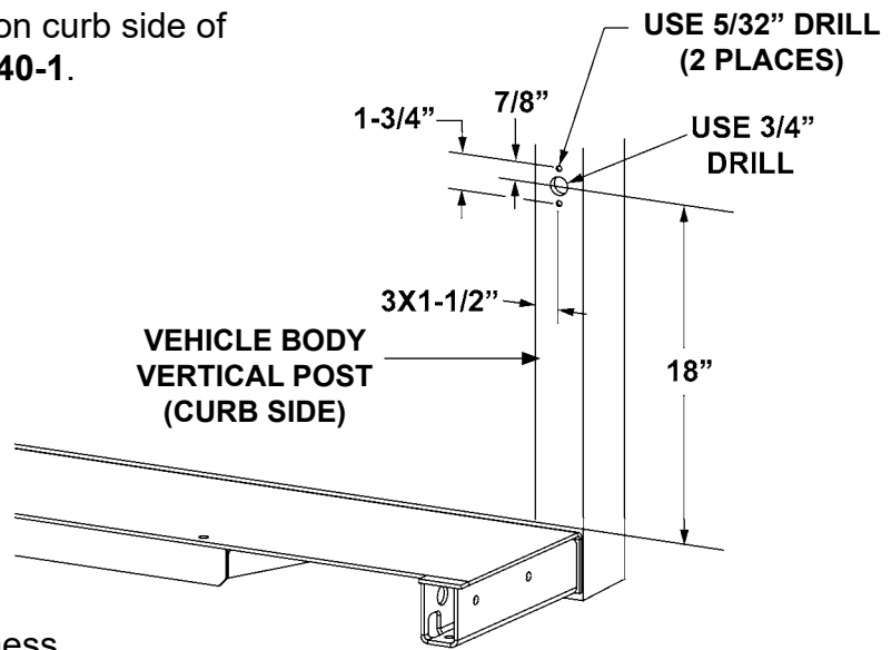
DRILLING MOUNTING HOLES FIG. 40-1
