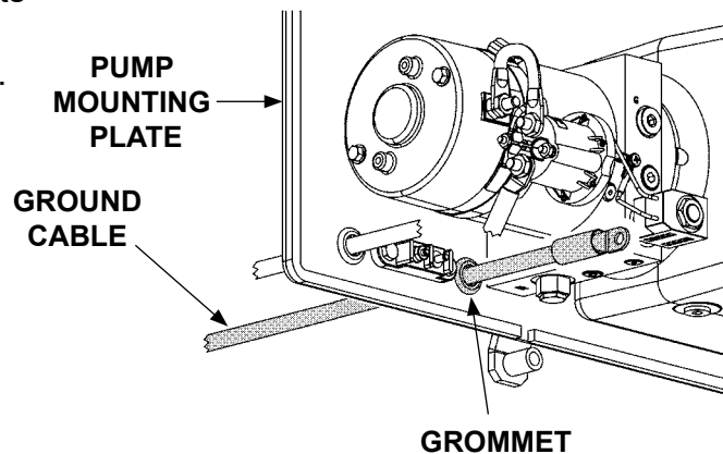
INSERTING GROUND CABLE THROUGH GROMMET FIG. 38-1
