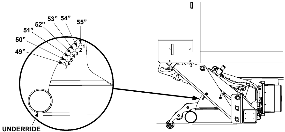
GPTLR-44 & GPTLR-55 CMVSS UNDERRIDE BRACKET SETTINGS BASED ON BED HEIGHT (RH BRACKET SHOWN) FIG. 68-1A
