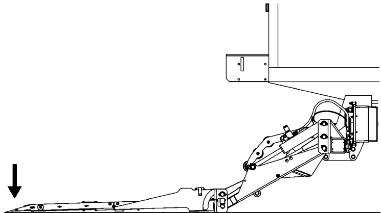
LOWERING PLATFORM FIG. 45-2
