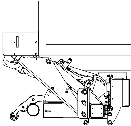
LIFTGATE WITH PLATFORM STOWED (STANDARD UNDERRIDE SHOWN ) FIG. 66-1
