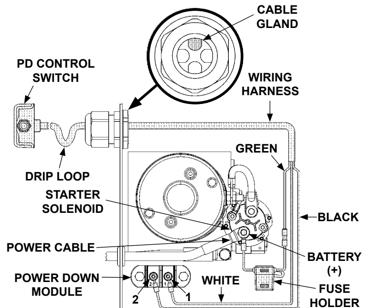
CONTROL SWITCH WIRING CONNECTIONS (POWER DOWN) FIG. 41-2
