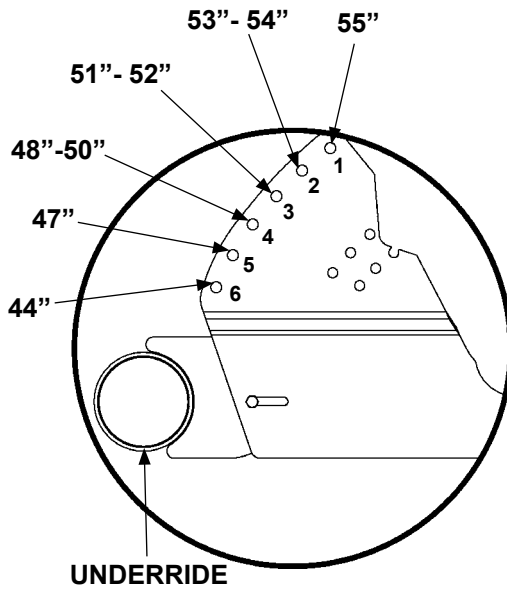
GPTLR-25 & GPTLR-33 FMVSS UNDERRIDE BRACKET SETTINGS BASED ON BED HEIGHT (RH BRACKET SHOWN) FIG. 67-1A
