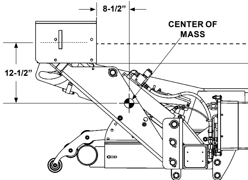
GPTLR-44 & GPTLR-55 CENTER OF MASS (STOWED POSITION) FIG. 15-2
