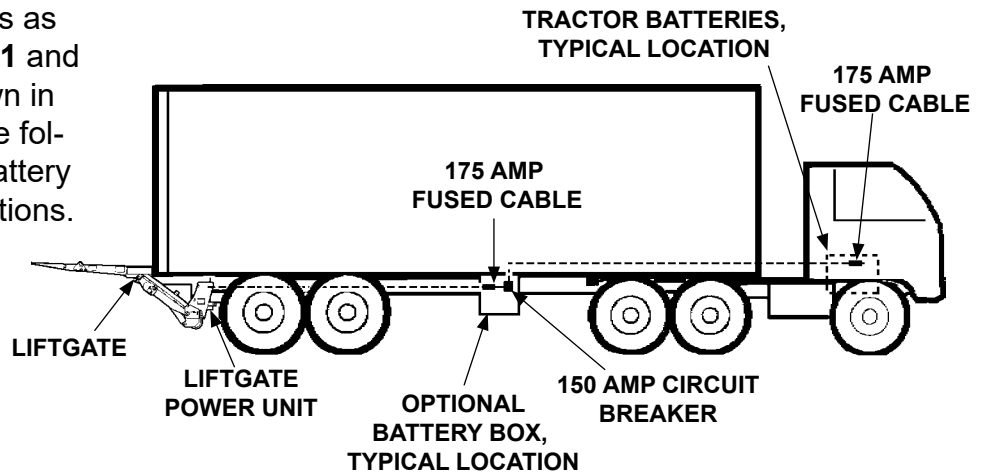
RECOMMENDED LIFTGATE & OPTIONAL BATTERY BOX INSTALLATION ON TRAILER FIG. 26-1
