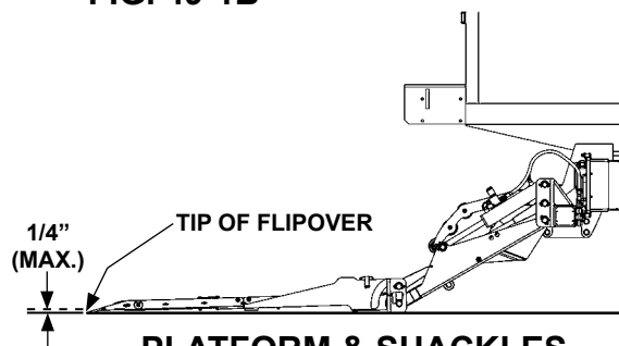
PLATFORM & SHACKLES TOUCH GROUND FIG. 49-2
