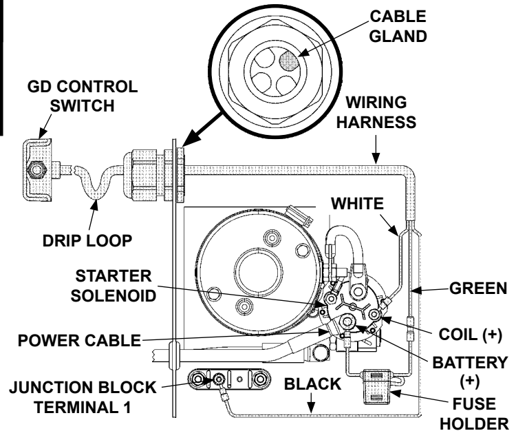
CONTROL SWITCH WIRING CONNECTIONS (GRAVITY DOWN) FIG. 41-1
