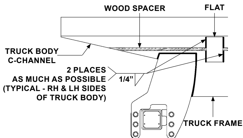
WELDING TRUCK BODY TO FRAME (RH SIDE SHOWN) FIG. 61-1
