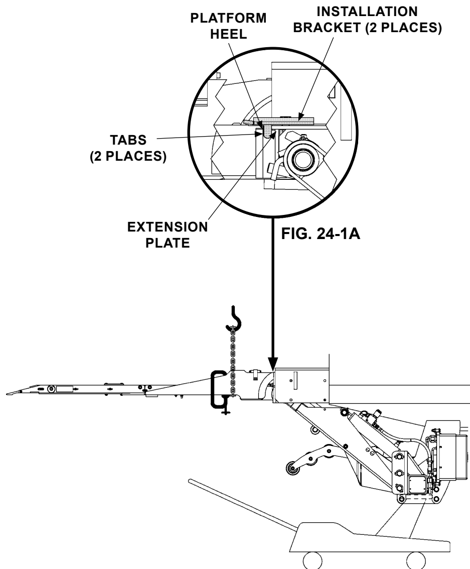
FITTING PLATFORM TIGHT AGAINST INSTALLATION BRACKET TABS FIG. 24-1
