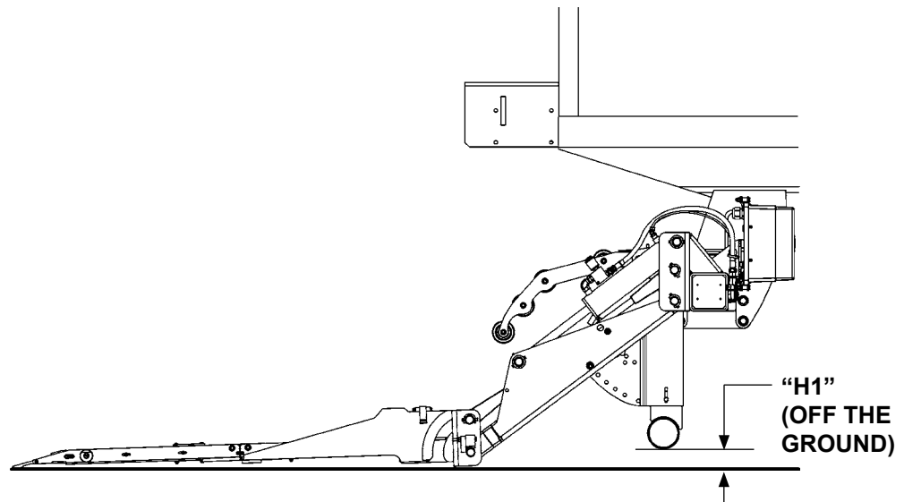
STANDARD FMVSS UNDERRIDE FIG. 73-2
