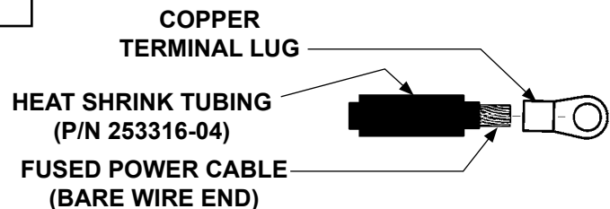
PLACING TERMINAL LUG & HEAT SHRINK TUBING ON FUSED POWER CABLE FIG. 36-2
