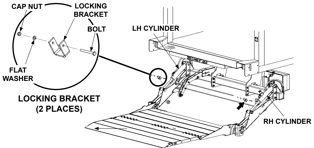
REMOVING LOCKING BRACKETS FIG. 46-1
