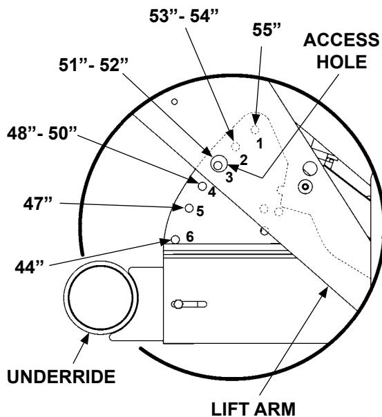
GPTLR-44 & GPTLR-55 FMVSS UNDERRIDE BRACKET SETTINGS BASED ON BED HEIGHT (RH BRACKET SHOWN) FIG. 67-2A
