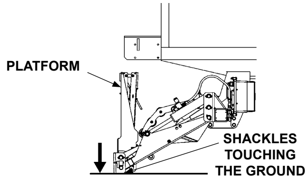
PLATFORM LOWERED FROM STOWED POSITION (RH SIDE VIEW) FIG. 62-1
