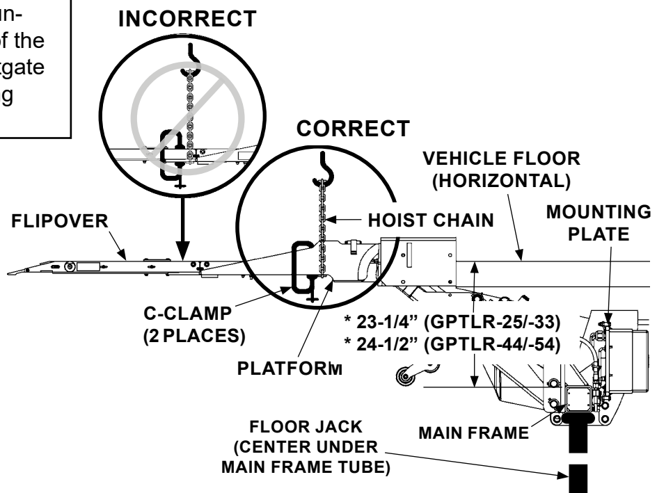
CORRECT WAY TO HOIST & SUPPORT LIFTGATE FIG. 23-1
