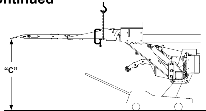
LIFTGATE CLEARANCE DIMENSIONS FIG. 56-1
