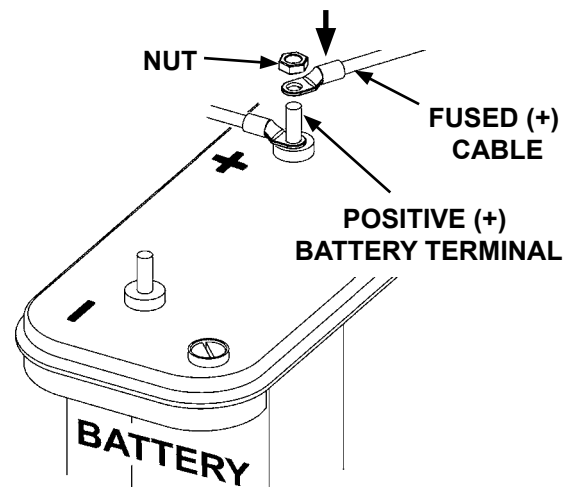
CONNECTING FUSED (+) CABLE FIG. 44-2
