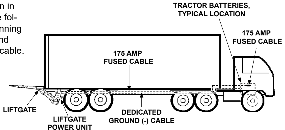
RECOMMENDED LIFTGATE & POWER CABLE INSTALLATION ON TRAILER
