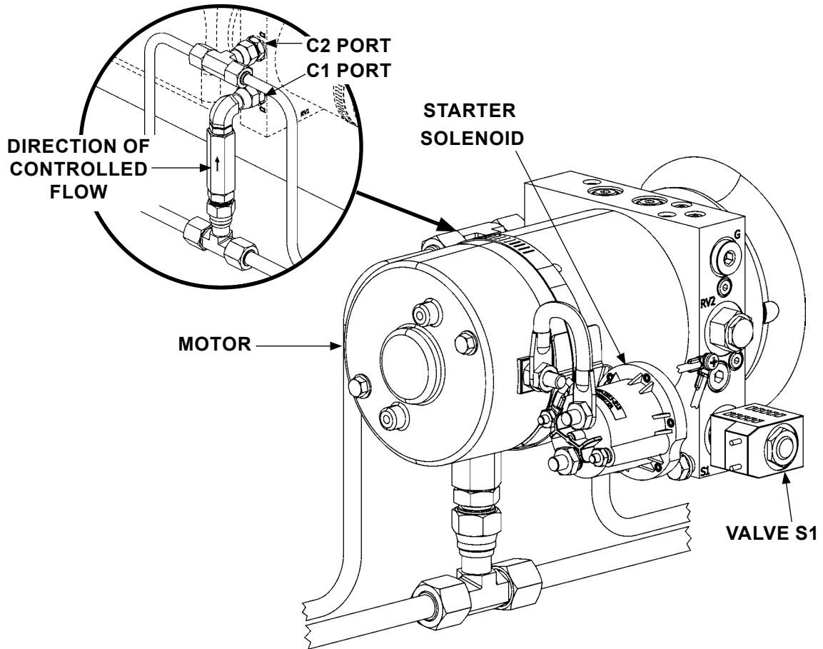
POWER DOWN POWER UNIT FIG. 85-1
