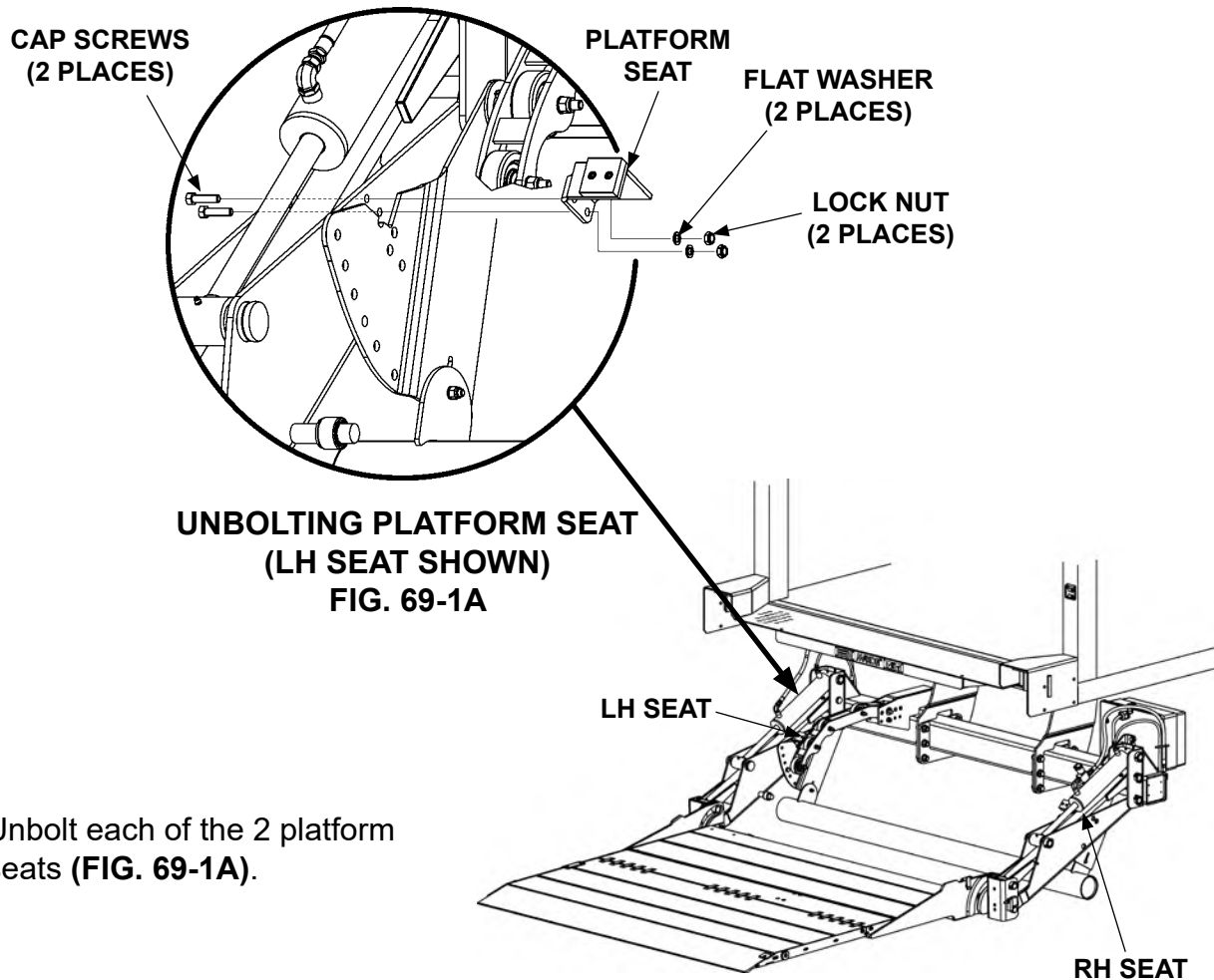
LIFTGATE WITH PLATFORM ON THE GROUND (STANDARD FMVSS UNDERRIDE SHOWN) FIG. 69-1
