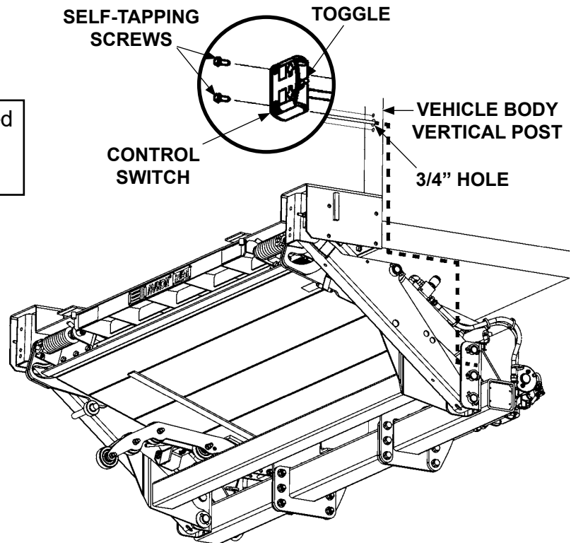
ROUTING CONTROL SWITCH WIRING FIG. 40-2
