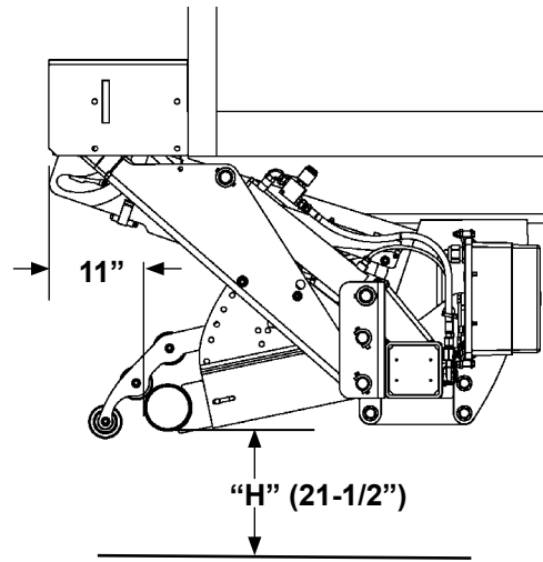
STANDARD FMVSS UNDERRIDE FIG. 73-1
