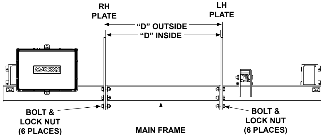
BOLT ON MOUNTING PLATES FOR INSTALLATION ON TRUCKS & TRAILERS (REAR VIEW OF LIFTGATE) FIG. 21-1
