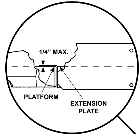
VERTICAL GAP FIG. 49-1A
