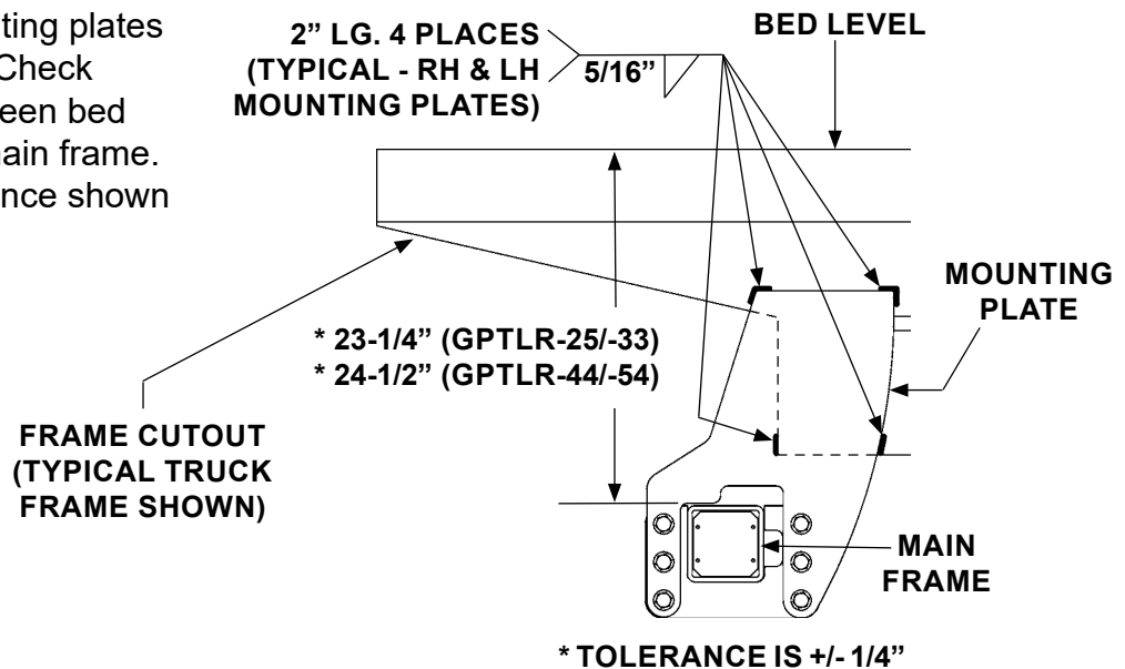
WELD TO VEHICLE FRAME AND MAIN FRAME (RH SIDE SHOWN) FIG. 25-1
