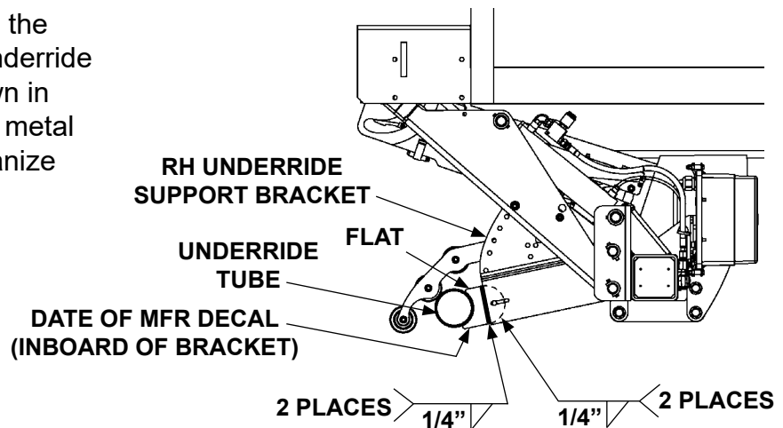
WELDING FLATS TO SUPPORT BRACKETS (RH SIDE SHOWN) FIG. 76-1
