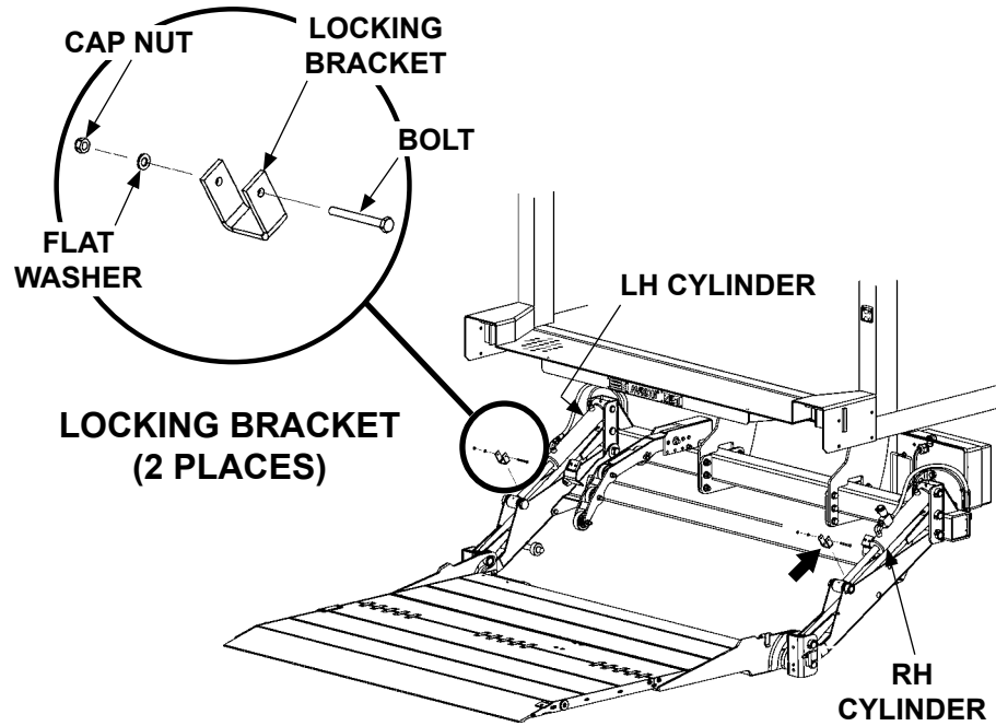
REMOVING LOCKING BRACKETS FIG. 59-1
