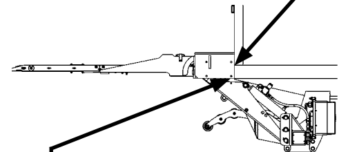
PLATFORM AT BED LEVEL FIG. 49-1
