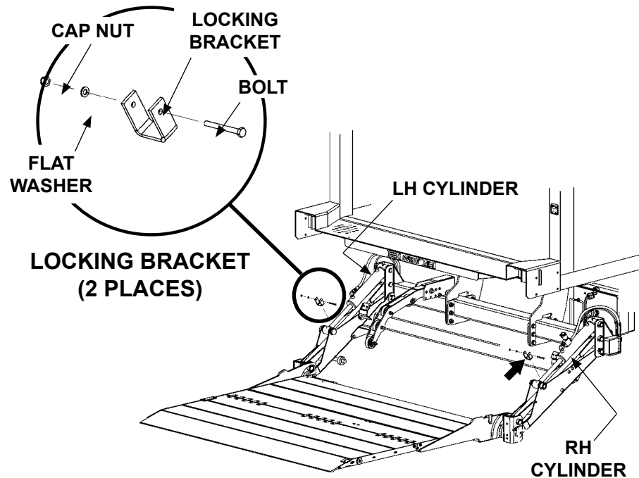
REINSTALLING LOCKING BRACKETS FIG. 53-1
