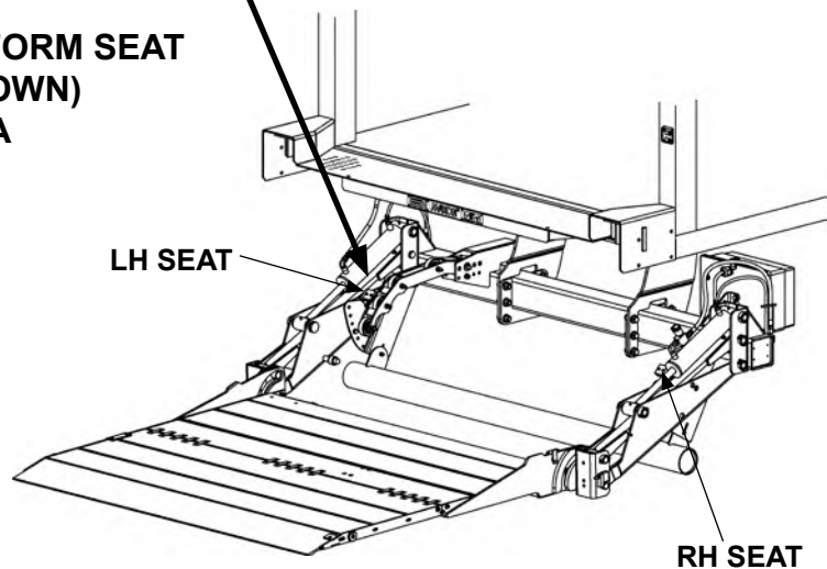
LIFTGATE WITH PLATFORM ON THE GROUND (STANDARD FMVSS UNDERRIDE SHOWN) FIG. 77-1
