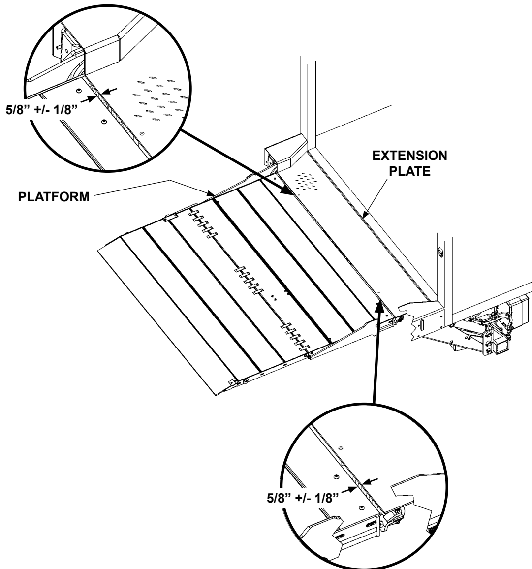
CHECKING GAP BETWEEN PLATFORM AND EXTENSION PLATE FIG. 48-1
