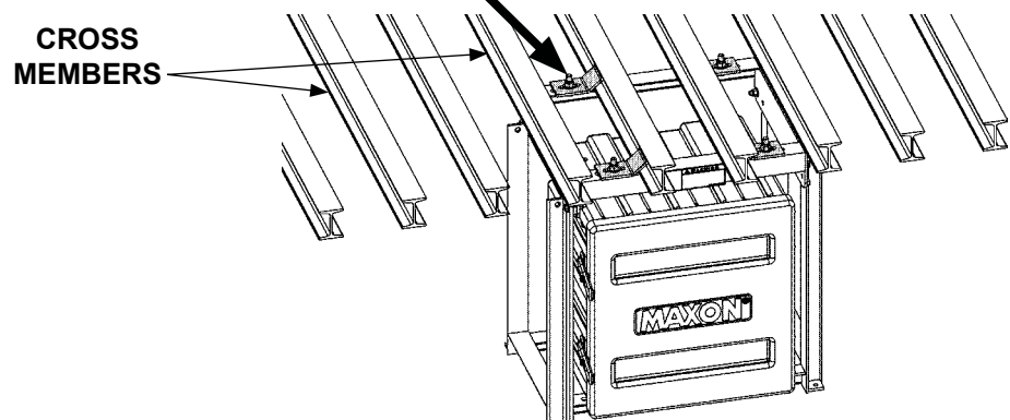
BOLTING BATTERY BOX FRAME FIG. 28-2
