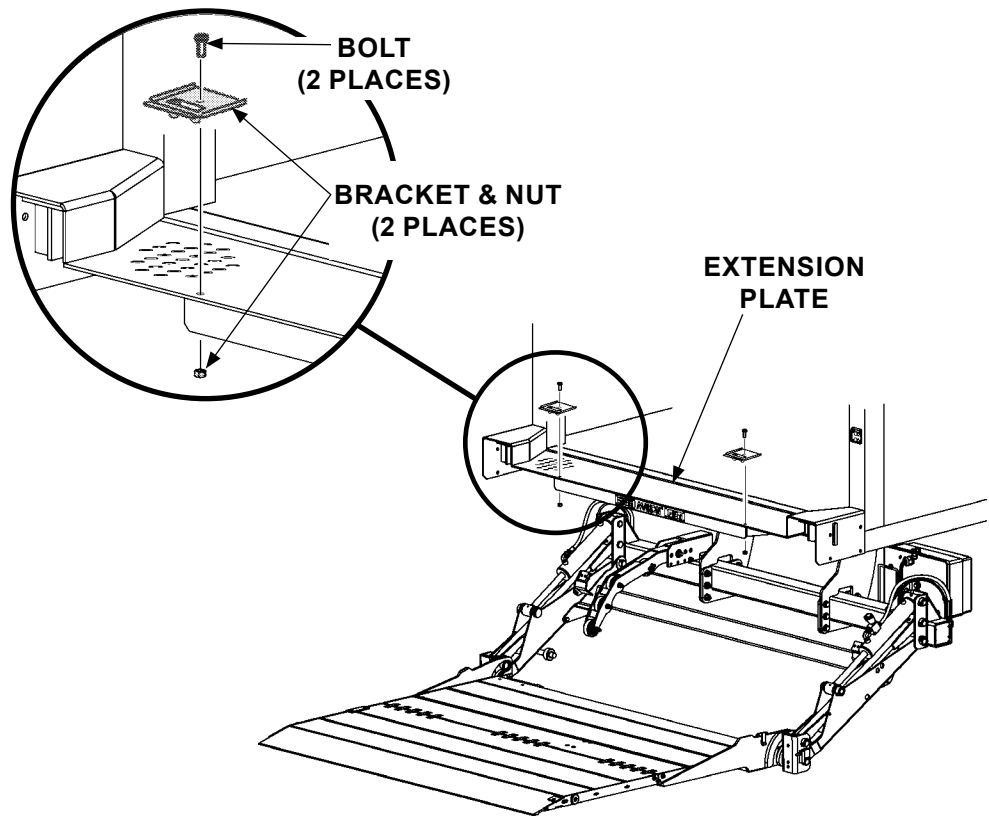
REINSTALLING INSTALLATION BRACKETS FIG. 52-1
