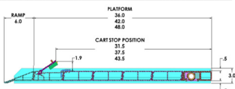
NEW DMD ONE PC PLATFORM WITH SINGLE OR DUAL CART STOP ON 9" RAMP
