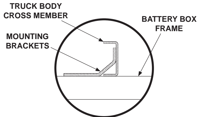
FLUSH BRACKETS FOR TRUCKS (8 PLACES) FIG. 24-2
