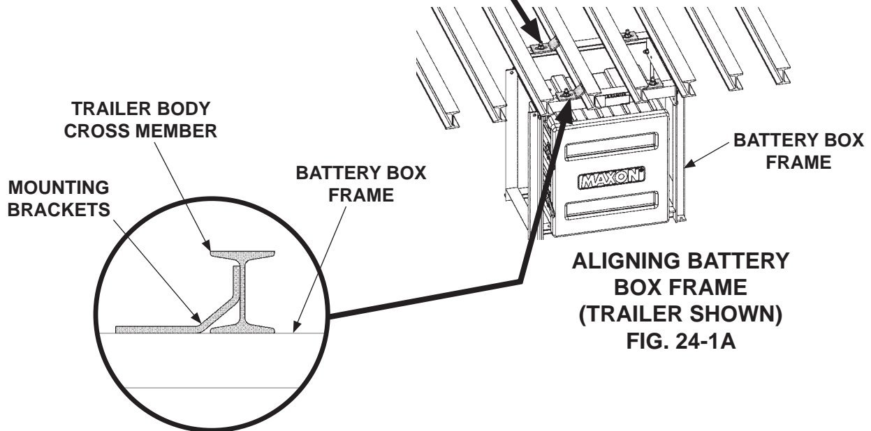
FLUSH BRACKETS FOR TRAILERS (8 PLACES) FIG. 24-1B
