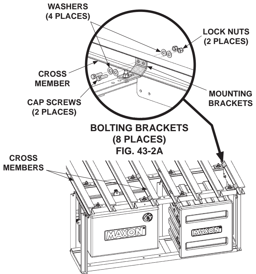
BOLTING PUMP & BATTERY BOX FRAME FIG. 43-2
