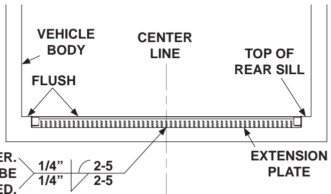
CENTERING EXTENSION PLATE ON 102" WIDE VEHICLE BODY FIG. 22-2
