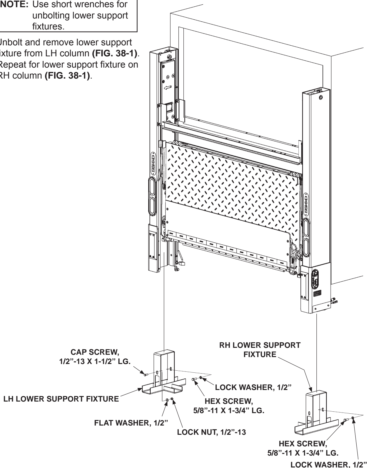
REMOVING LOWER SUPPORT FIXTURES
