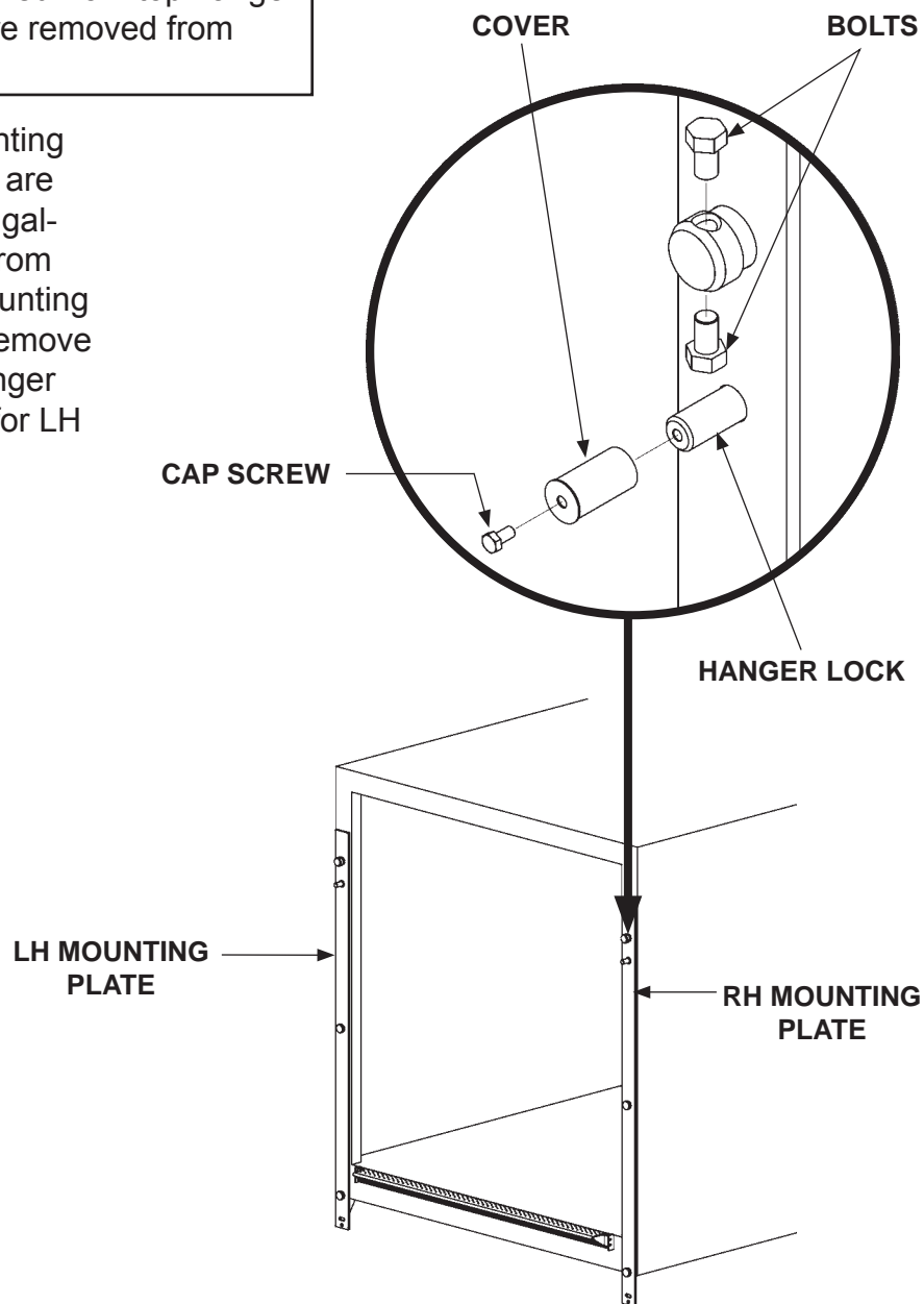
LIFTGATE MOUNTING PLATES FIG. 34-1
