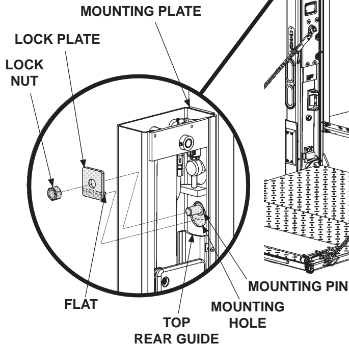
INSTALLING LOCK PLATE (LH COLUMN SHOWN) FIG. 73-1A
