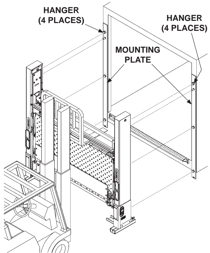
HANGING LIFTGATE FIG. 35-1
