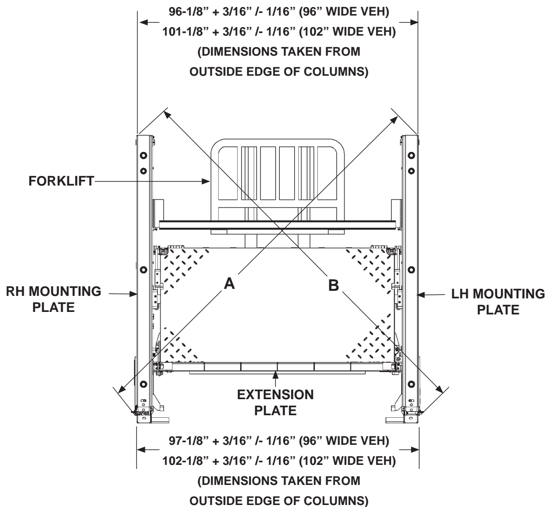
CHECKING IF COLUMNS ARE SQUARE (REAR OF LIFTGATE SHOWN) FIG. 28-1
